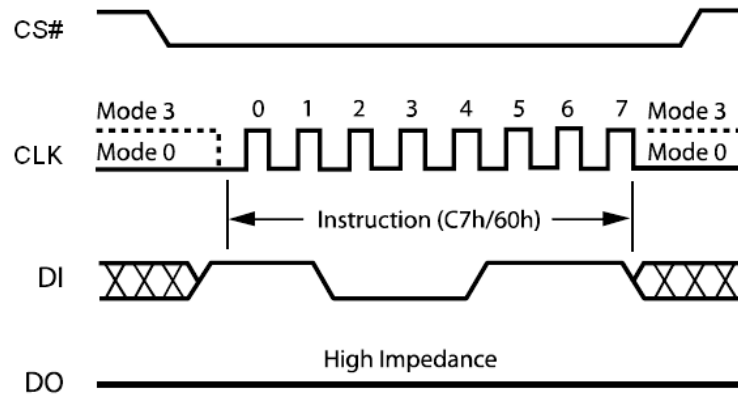
Figure 23. Chip Erase Instruction Sequence Diagram
