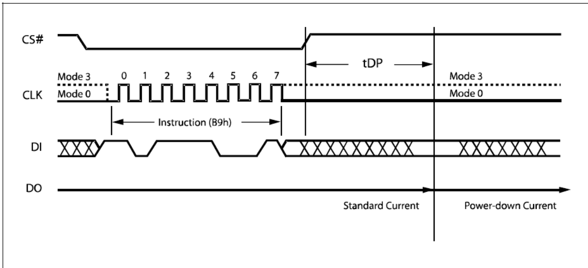
Figure 24. Deep Power-down Instruction Sequence Diagram
