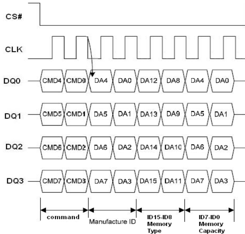
Figure 28.1. Read Identification (RDID) in QPI Mode
