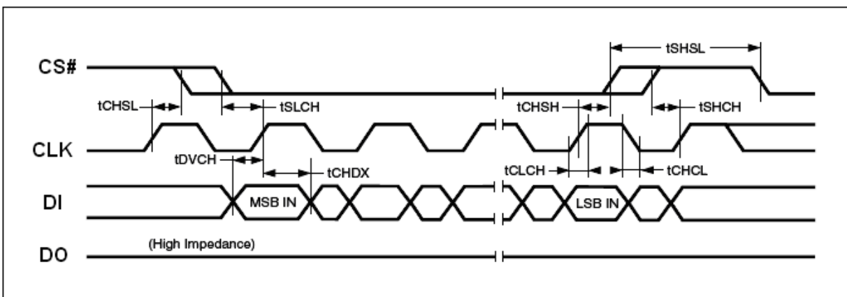
Figure 34. Input Timing
