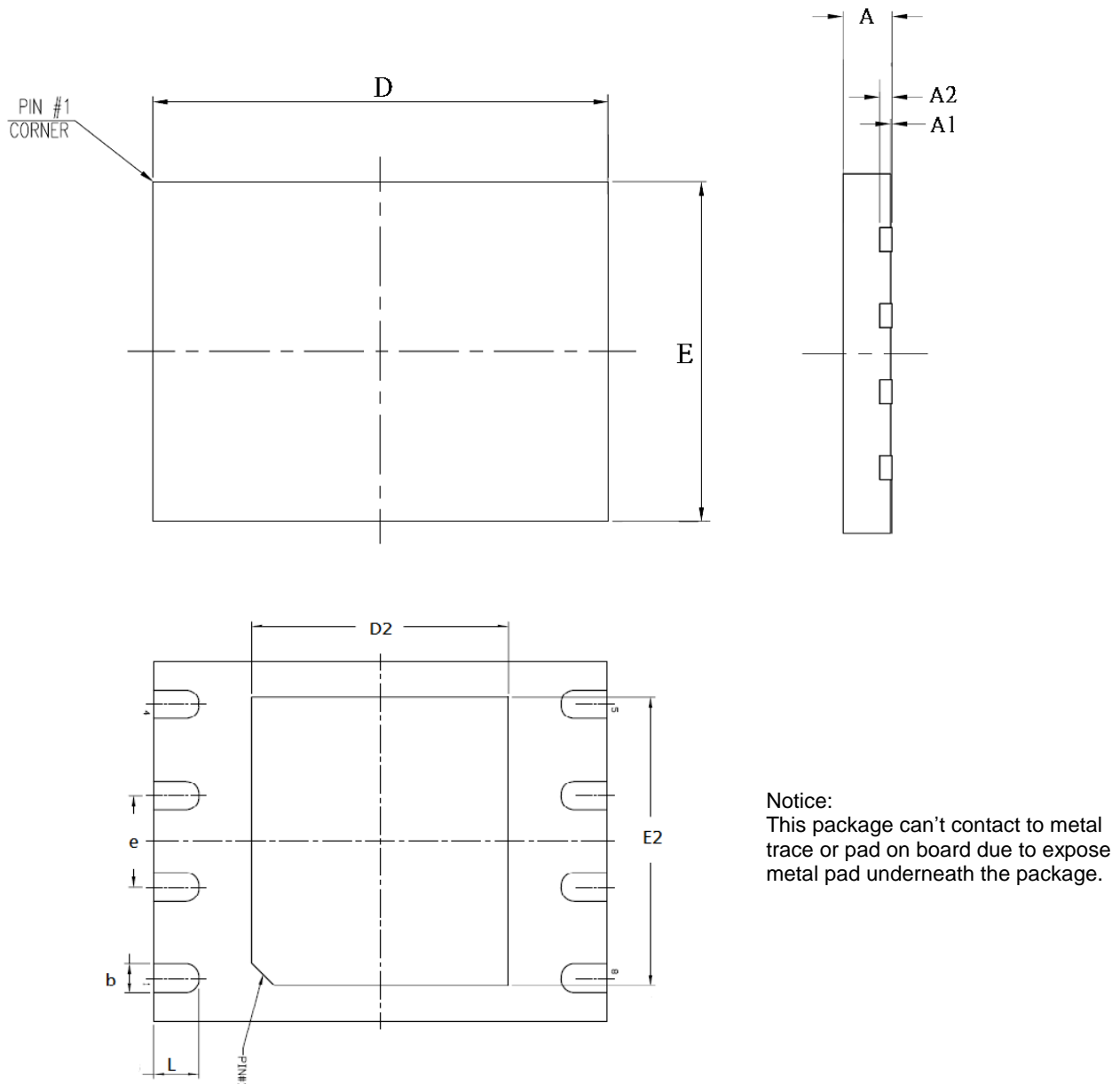
Figure 39. VDFN/ WSON 8 (6x5mm )
