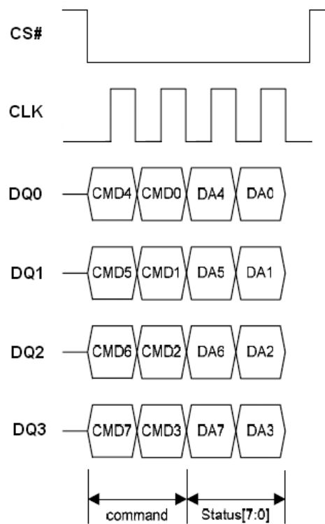
Figure 12.1 Write Status Register Instruction Sequence in QPI Mode
