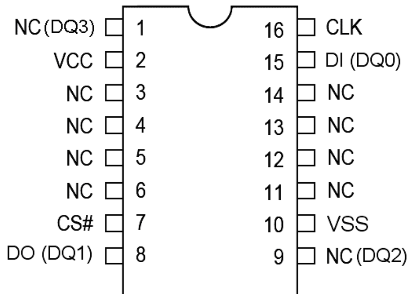
16 - LEAD SOP
