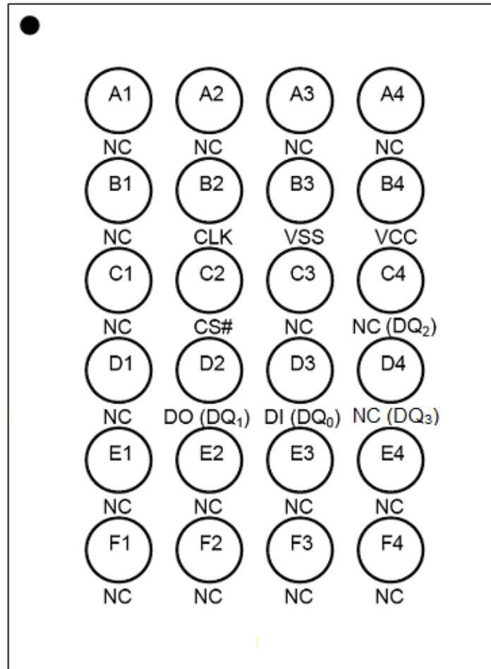
24 - Ball TFBGA
