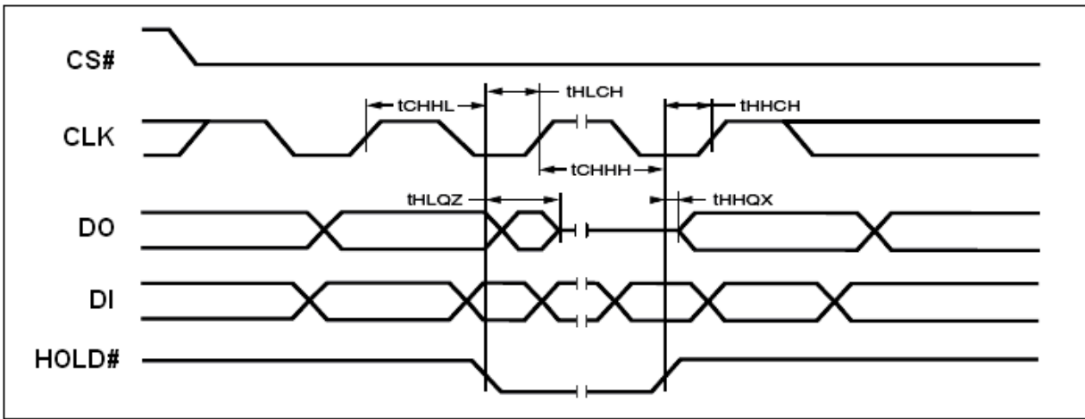
Figure 39. Hold Timing
