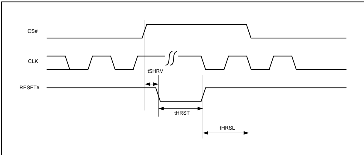
Figure 40. Reset Timing
