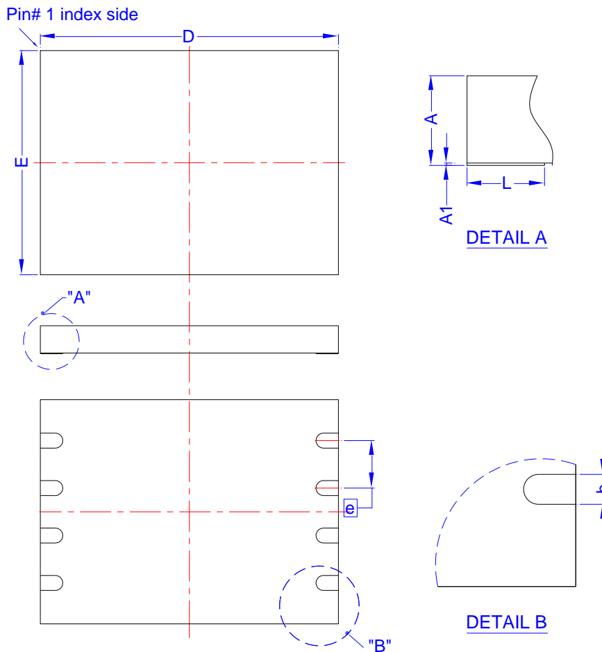
Figure 47. VDFN / WSON 8 ( 8x6mm ) without Expose metal pad
