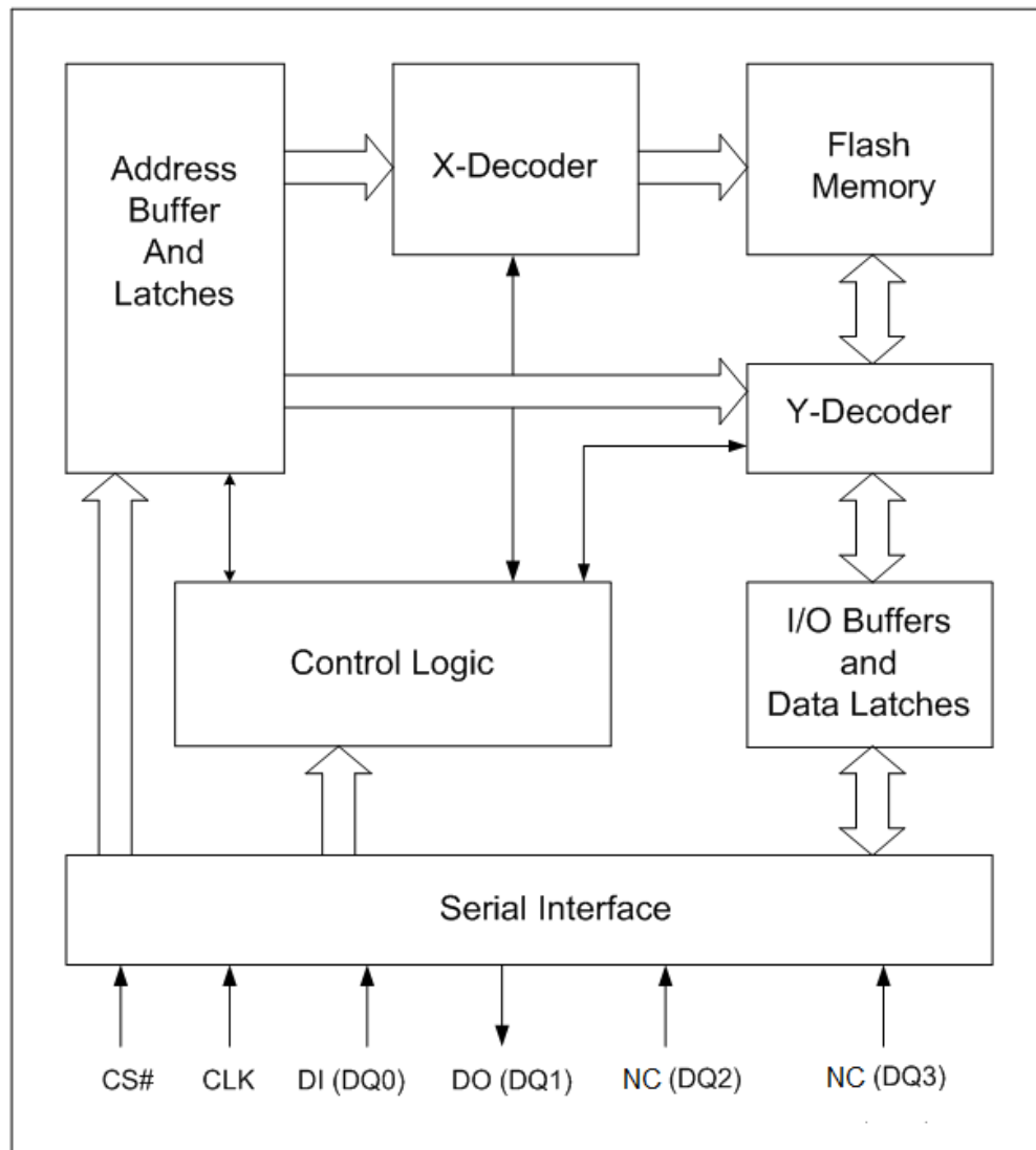
Figure 2. BLOCK DIAGRAM
