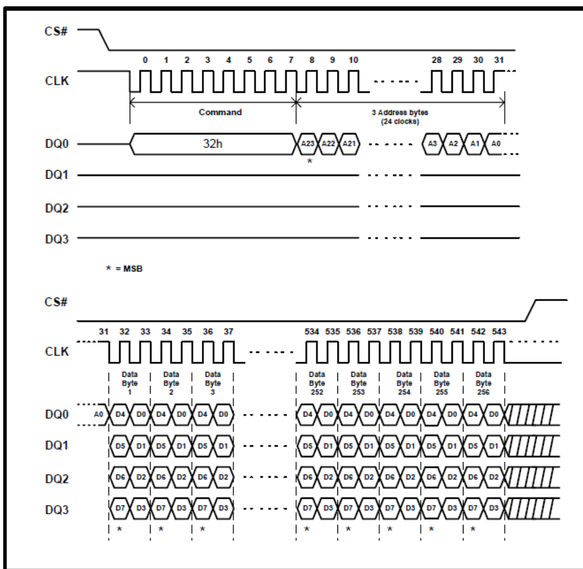
Figure 26. Quad Input Page Program Instruction Sequence Diagram (SPI Mode only)
