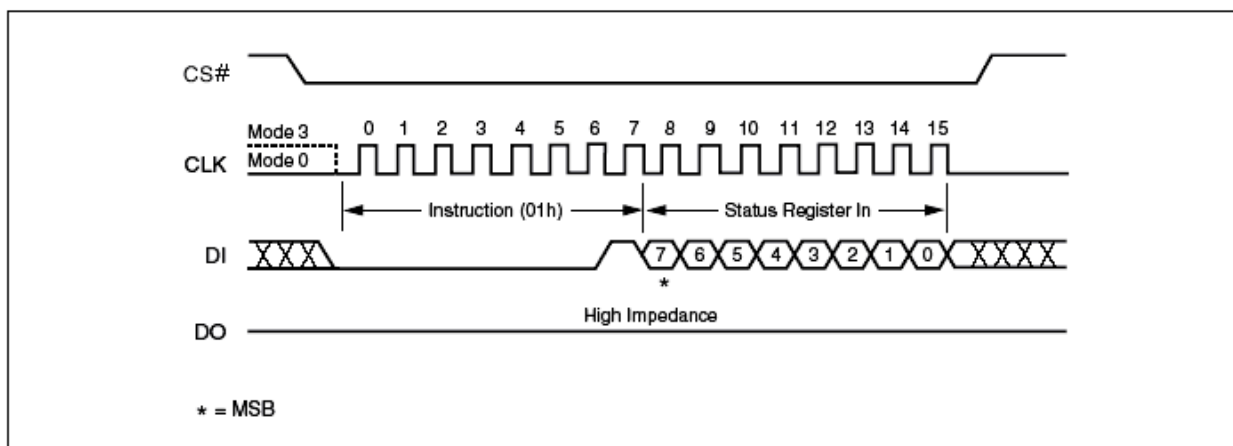
Figure 15. Write Status Register Instruction Sequence Diagram
