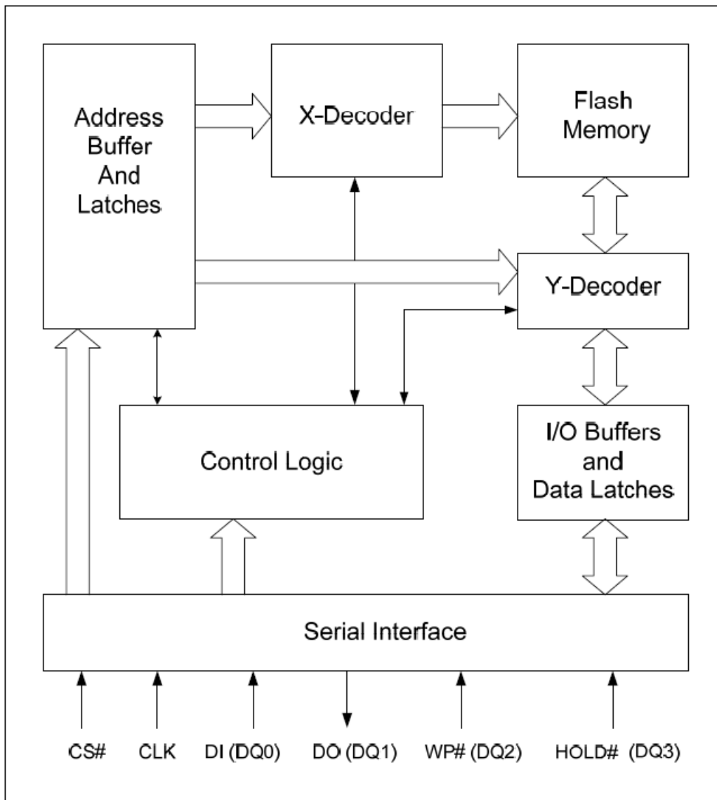
Figure 2. BLOCK DIAGRAM
