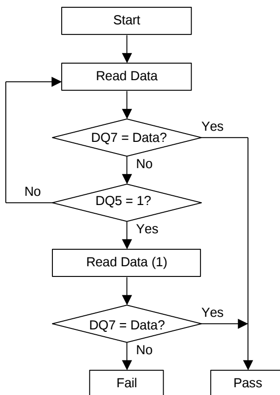
Flowchart 5. DATA# Polling Algorithm
