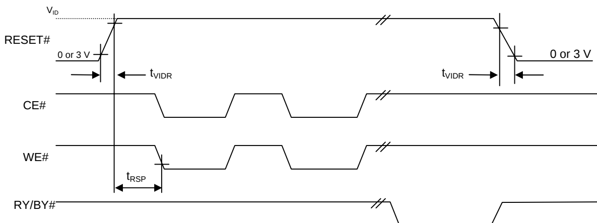
Figure 11. Temporary Sector Unprotect Timing Diagram
