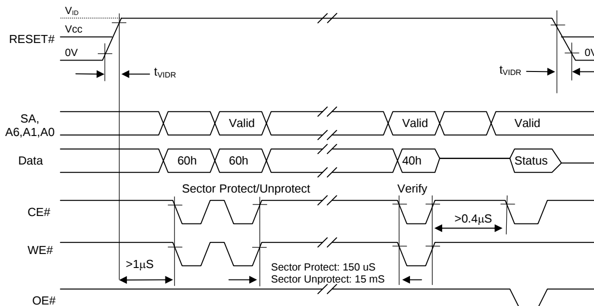
Figure 10. Sector Protect/Unprotect Timing Diagram
