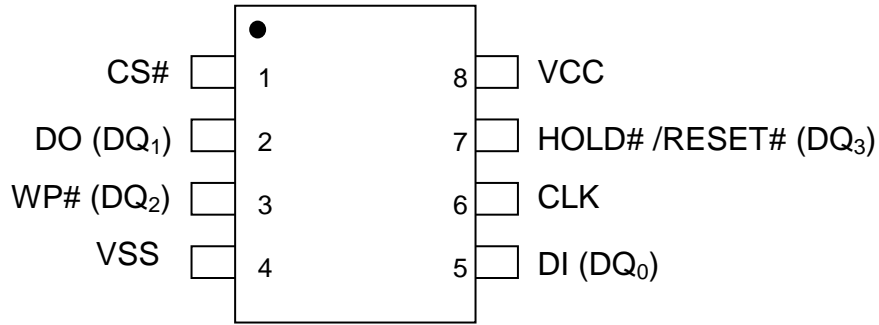
8 - LEAD SOP
