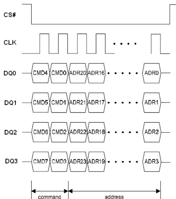
Figure 78. Erase OTP array (QPI mode)
