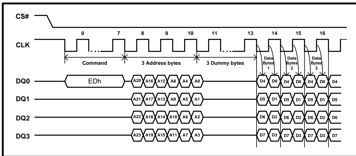
Figure 36. DDR Quad Input / Output FAST_READ Instruction Sequence Diagram
