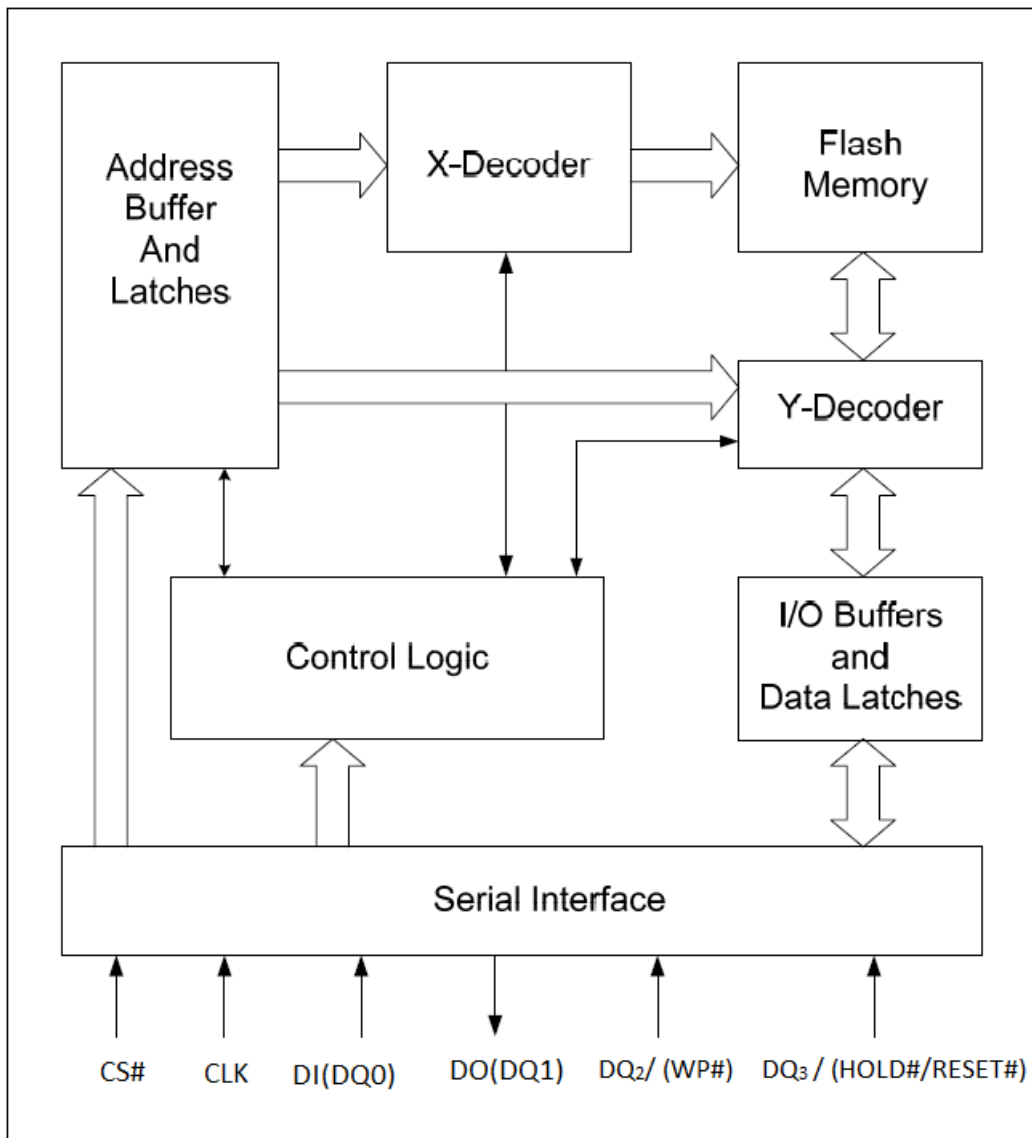
Figure 1. BLOCK DIAGRAM
