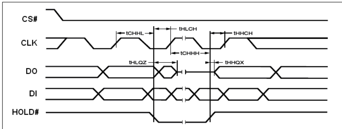
Figure 90. Hold Timing
