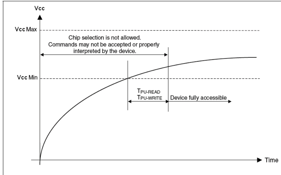
Figure 86. Power-up Timing
