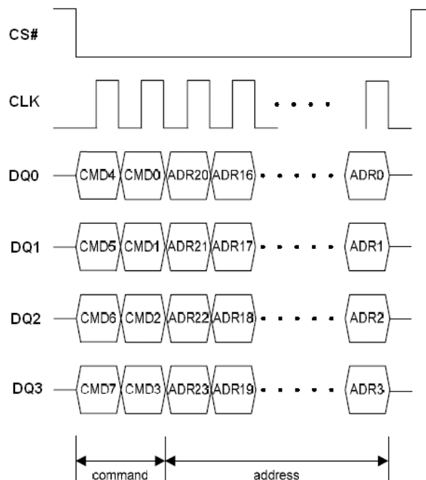
Figure 61. Block / Sector Erase Instruction Sequence in QPI Mode
