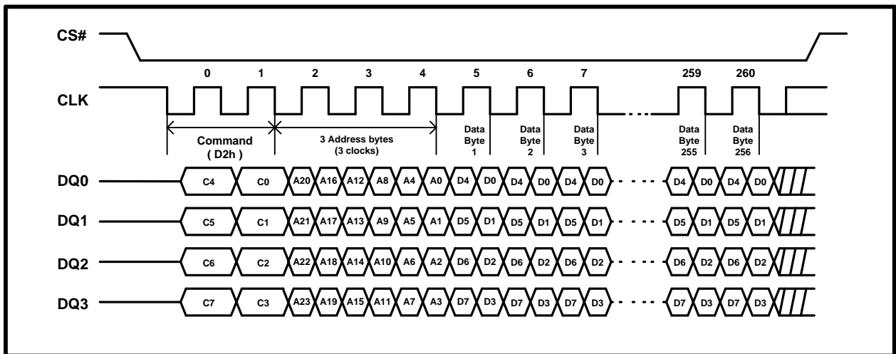
Figure 50. DDR Page Program Instruction Sequence Diagram in QPI Mode
