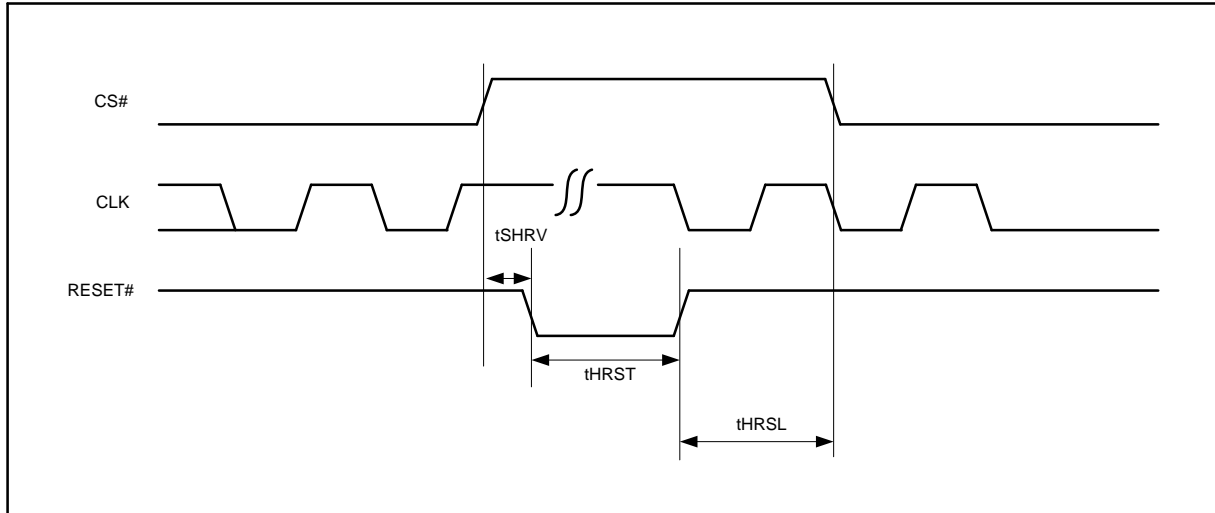
Figure 91. Reset Timing
