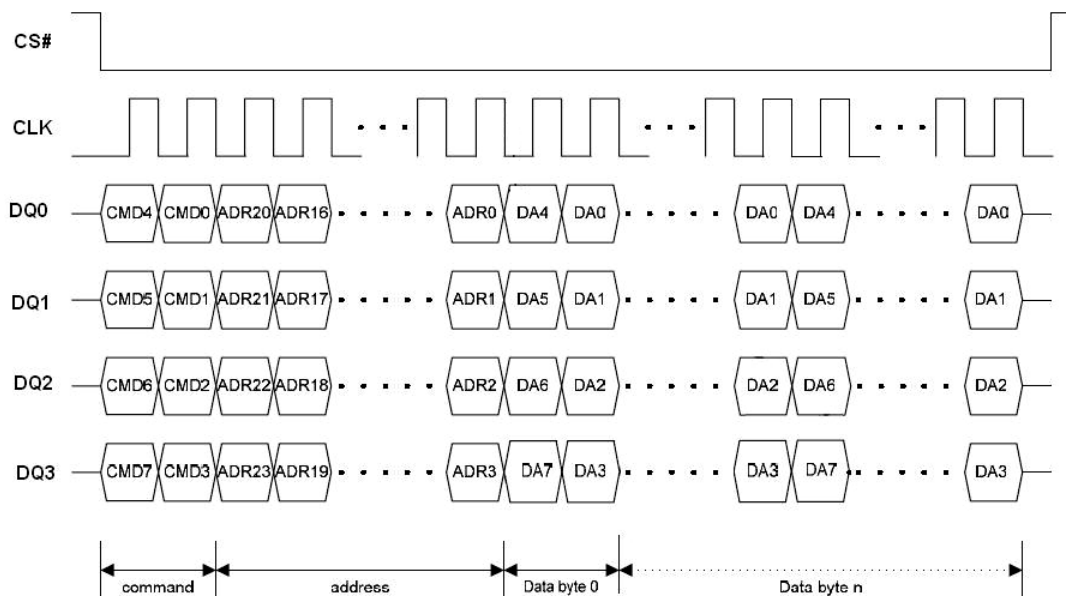
Figure 4. Full Quad SPI Modes
