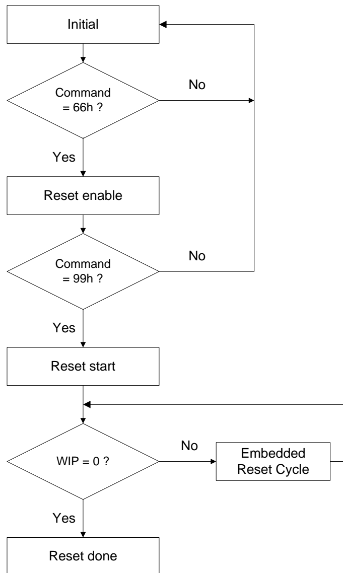
Figure 7. Software Reset Flow
