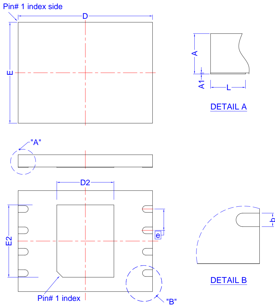
Figure 98. 8-LEAD VDFN / WSON (8x6 mm)
