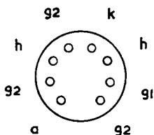
B8D BASE (10mm. subminiature)
