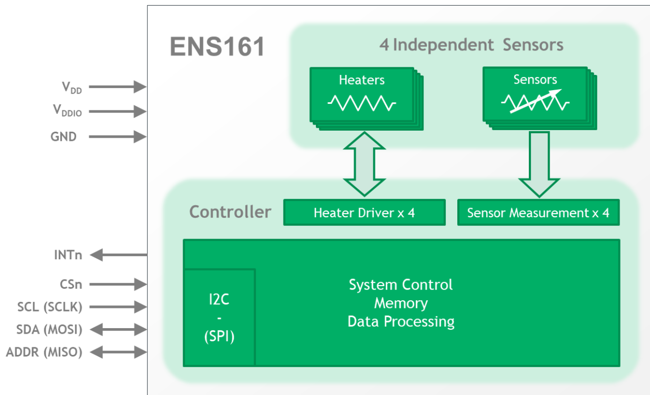
Figure 1: Functional Blocks
