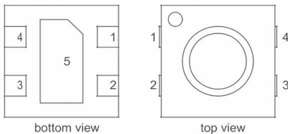
Figure 3: Pin diagram
