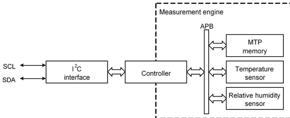
Figure 2: Functional blocks
