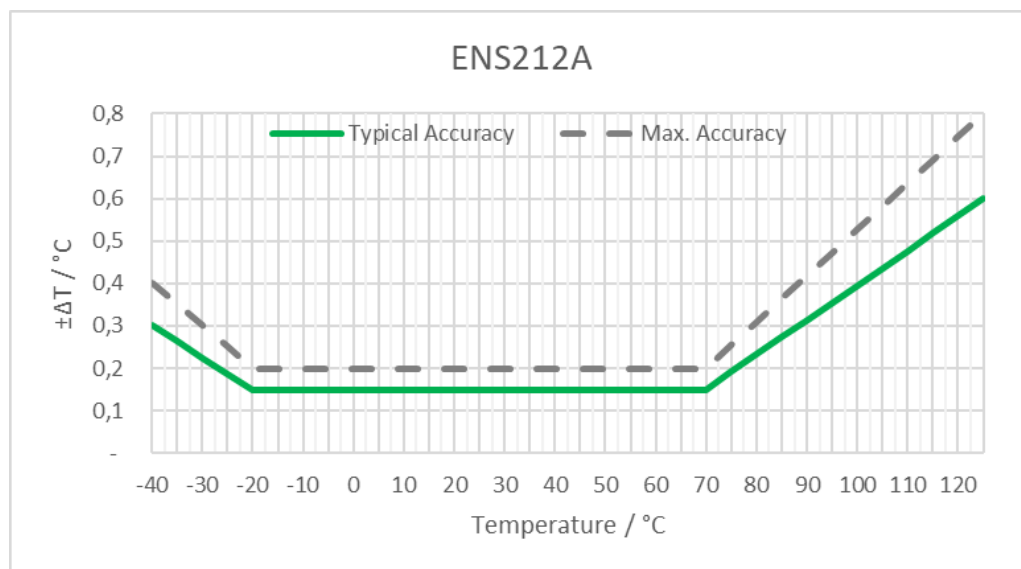
Figure 6: Temperature sensor accuracies
