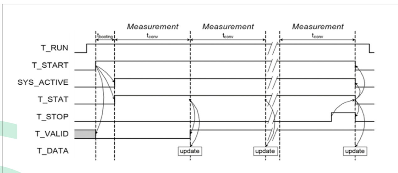
Figure 13: Continuous temperature measurement
