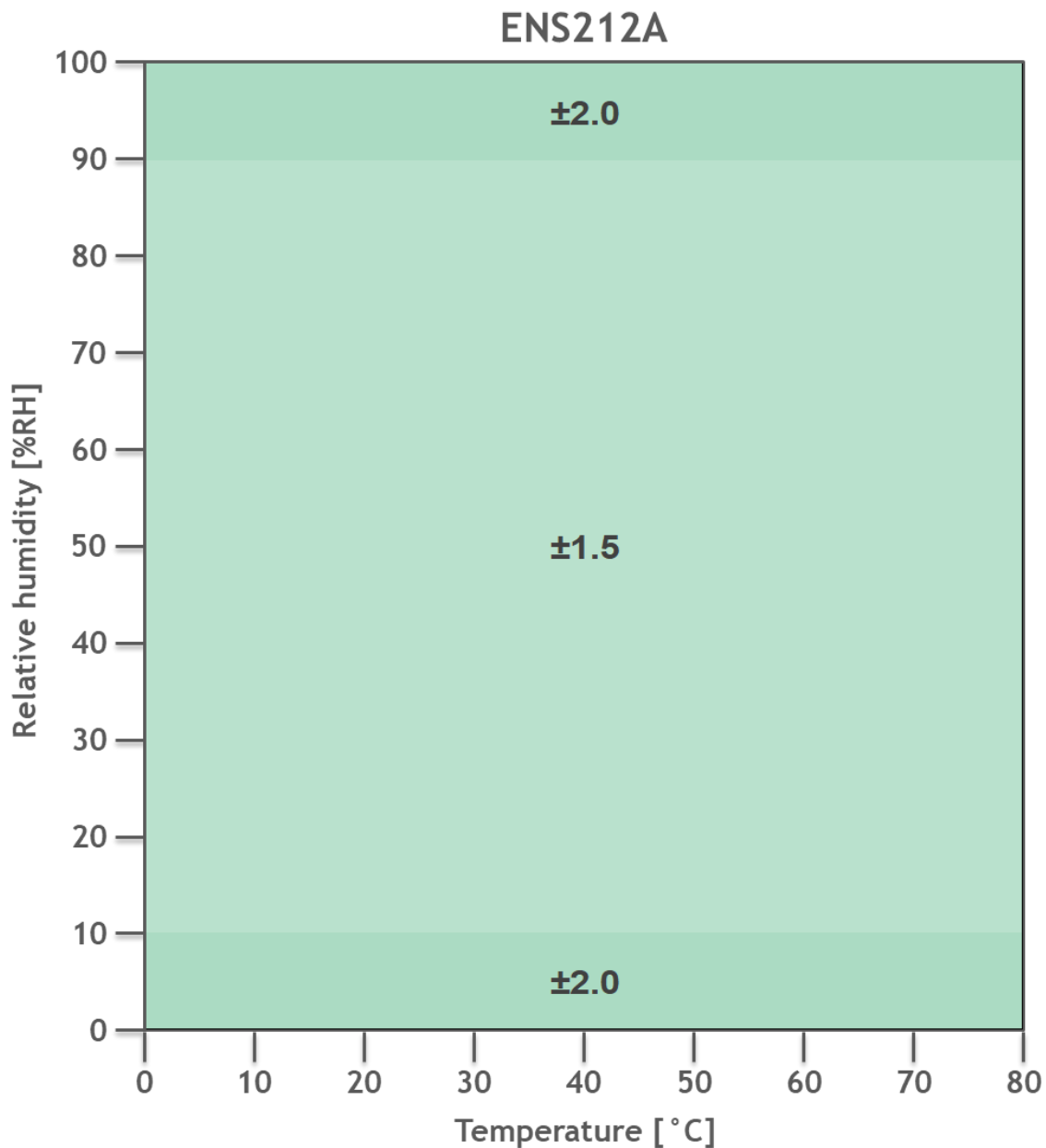
Figure 9: Accuracy of relative humidity measurements (%RH) as function of temperature and relative humidity 11
