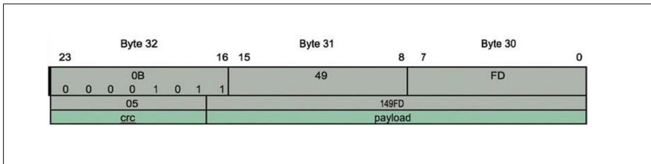
Figure 15: T_VAL readout
