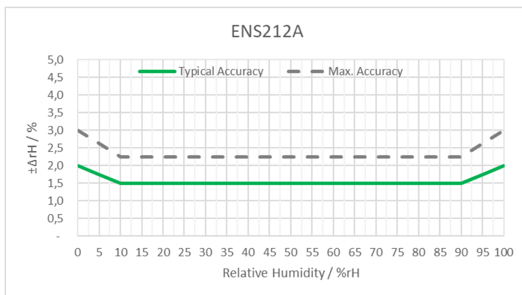
Figure 8: Relative humidity sensor accuracies 10
