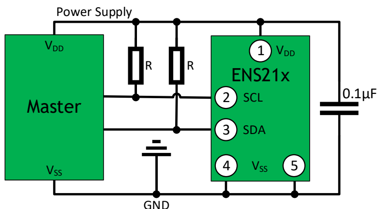
Figure 16: ENS212A typical application
