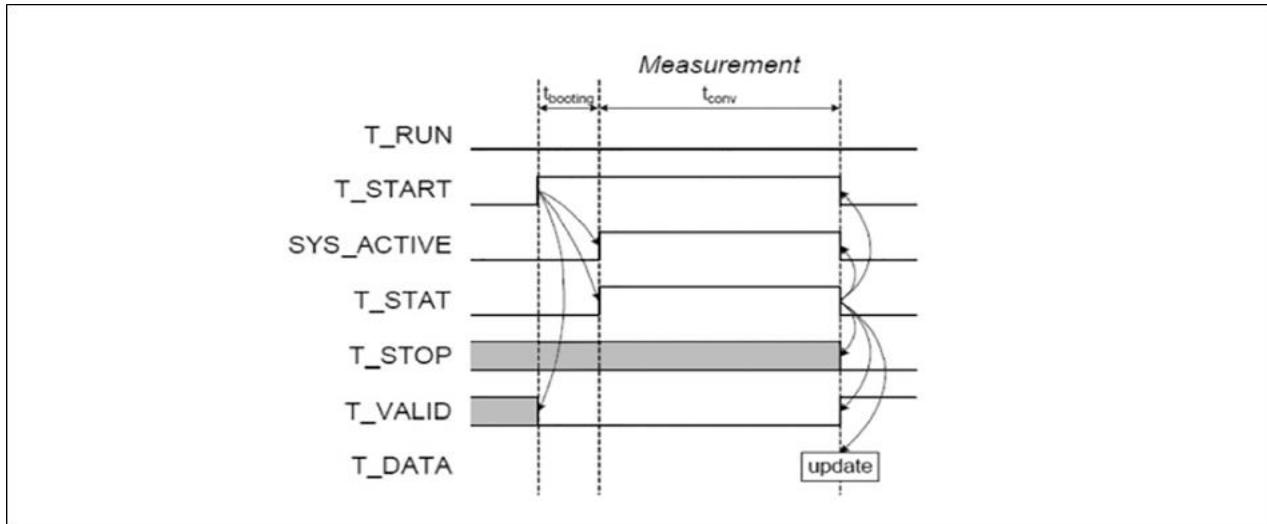
Figure 12: Single shot temperature measurement
