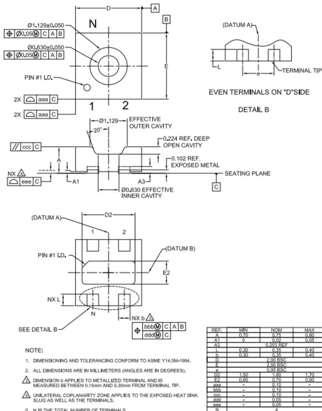
Figure 20: Package outline
