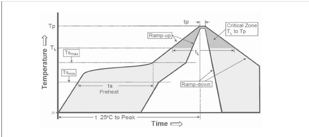
Figure 18: Soldering recommendations
