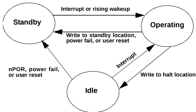
Figure 3. State Diagram
