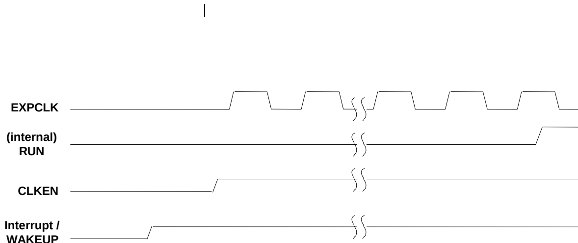
Figure 5. CLKEN Timing Entering the Standby State
