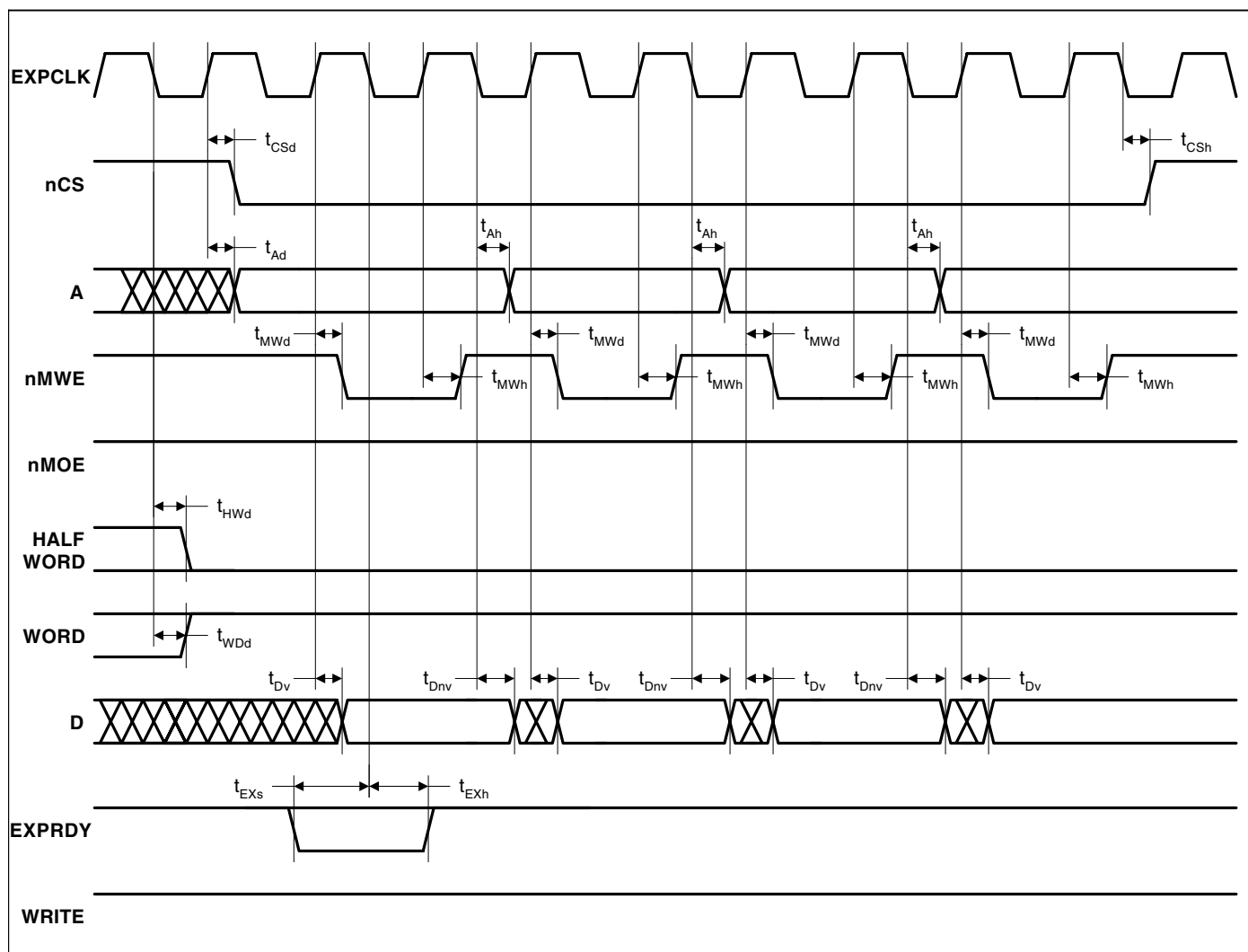
Figure 5. Static Memory Burst Write Cycle Timing Measurement
