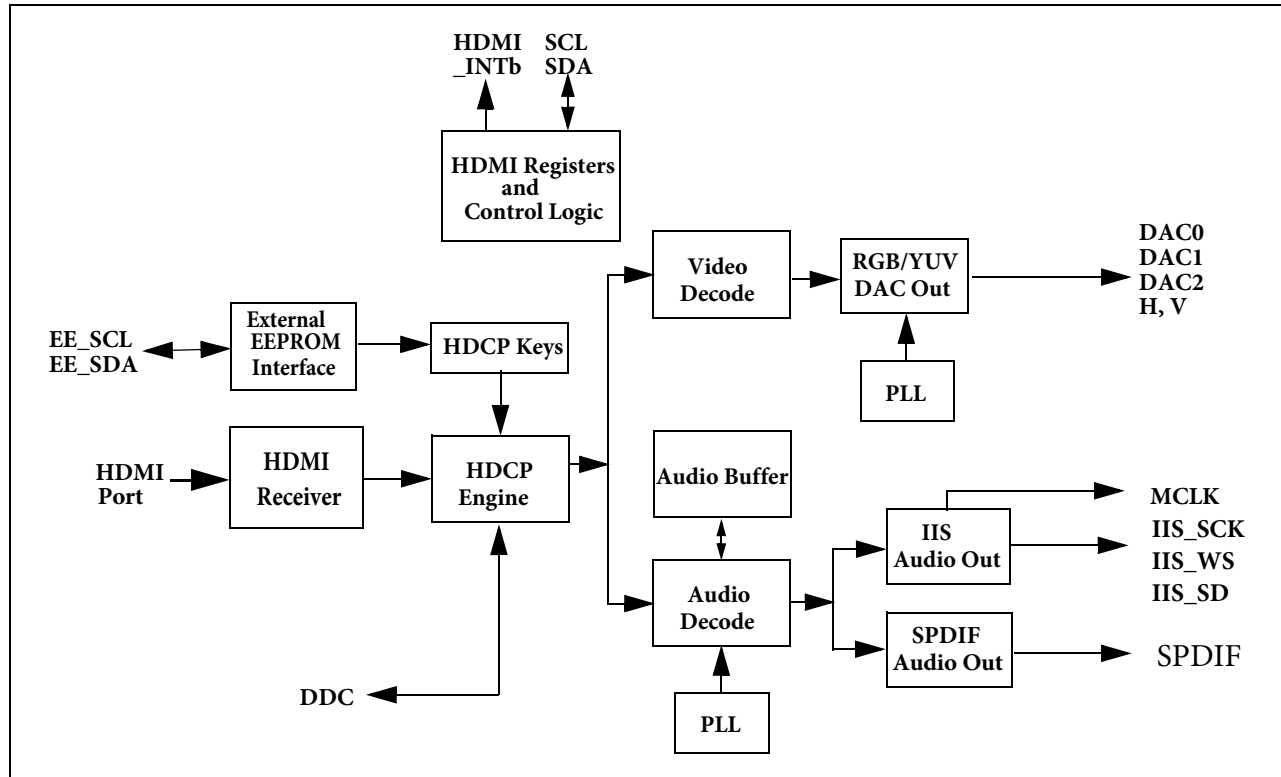
Figure 2-1 Block Diagram
