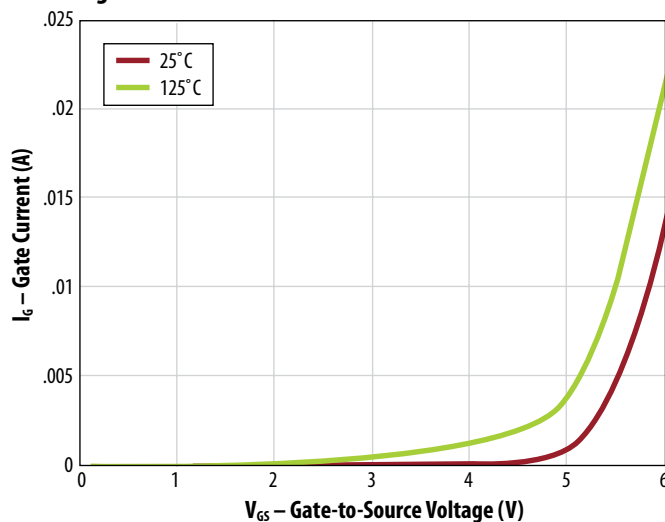
Figure 10: Gate Current
