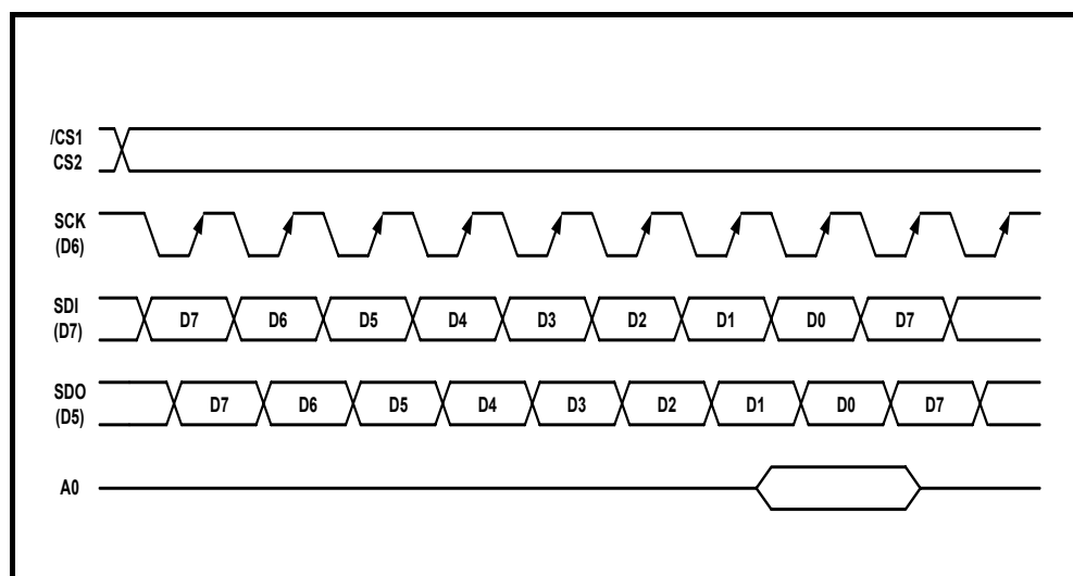
Figure 4 Serial Interface Signal Chart
