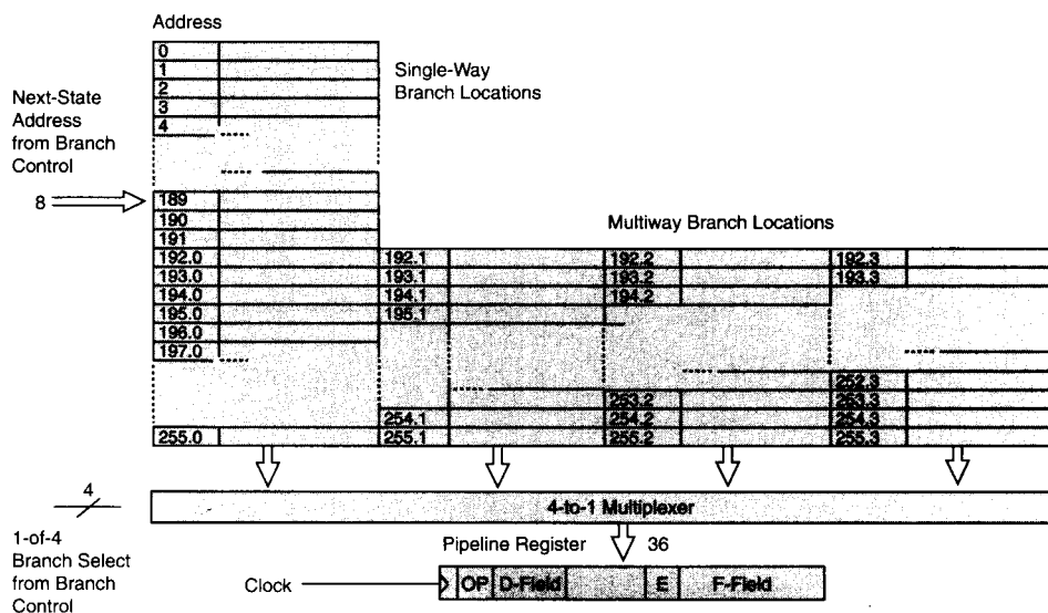
Figure 3. Microcode Memory
