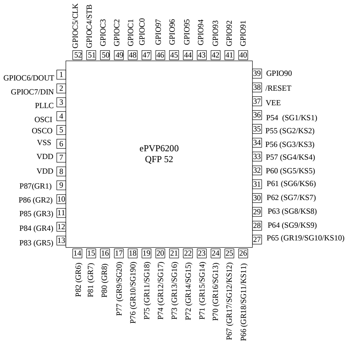
Fig. 1 Pin Assignment
