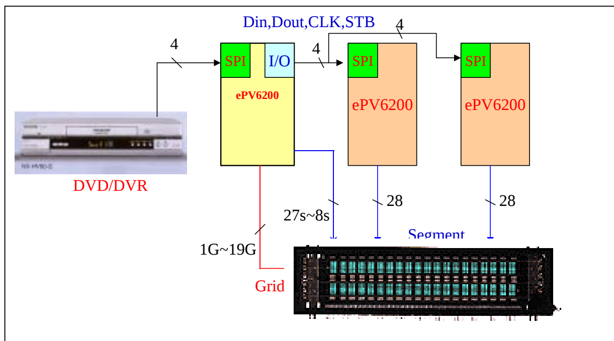
Fig. 25 Block Diagram for Cascade Application
