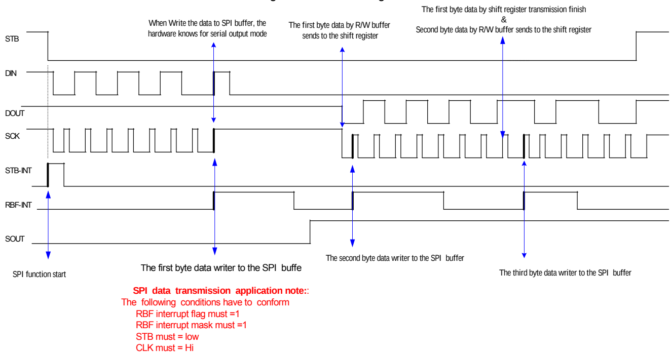
Fig. 4b SPI Timing Diagram
