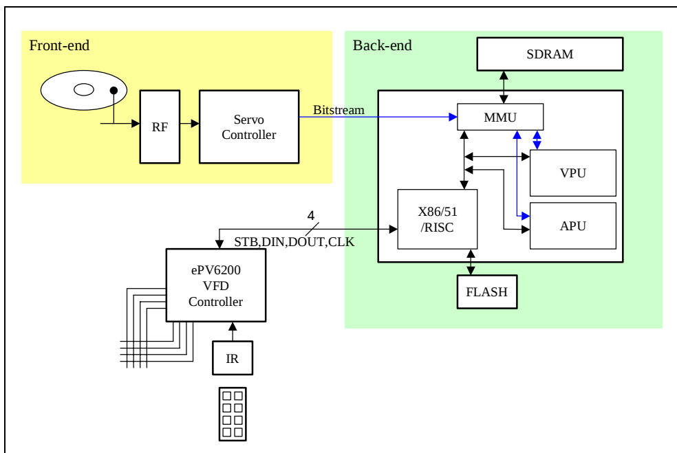
Fig. 24 Block Diagram for DVD Player Application
