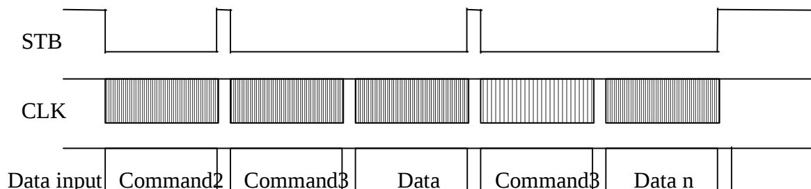
Fig. 23 Specific Address Timing Diagram
