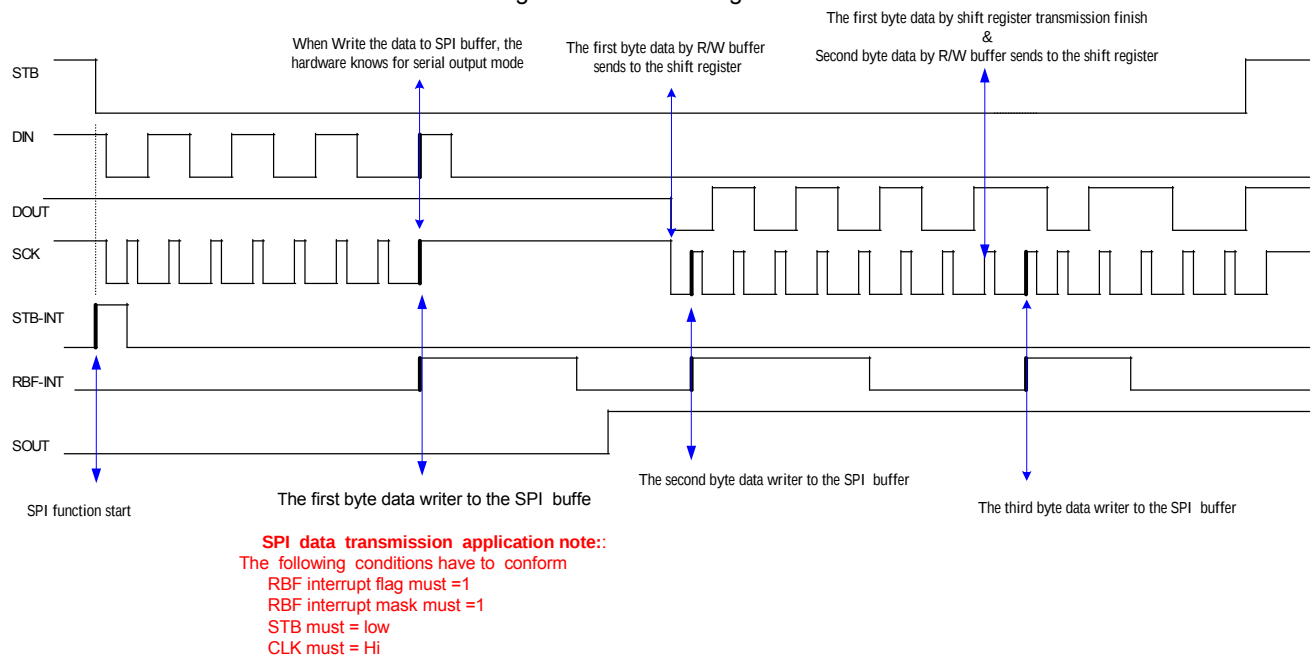
Fig. 4b SPI Timing Diagram
