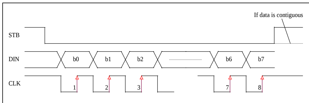
Fig. 19 Data Reception Timing Diagram
