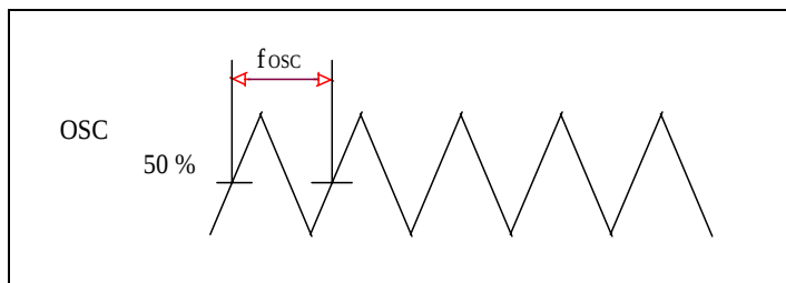
Fig. 21a Switching Characteristic Waveform
