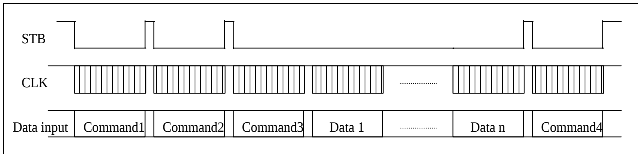
Fig. 22 incrementing Address Timing Diagram
