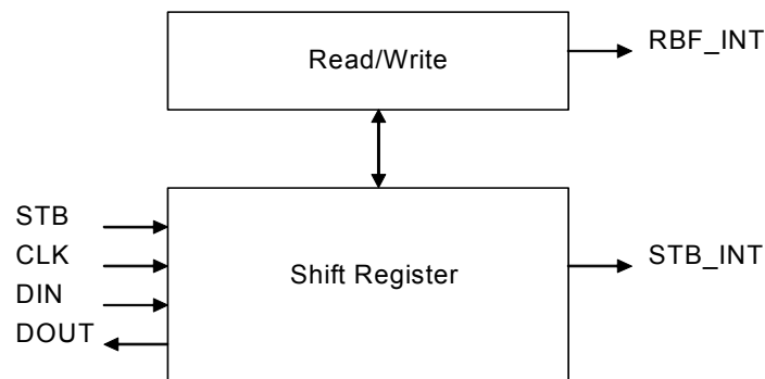
Fig. 4a SPI Block Diagram
