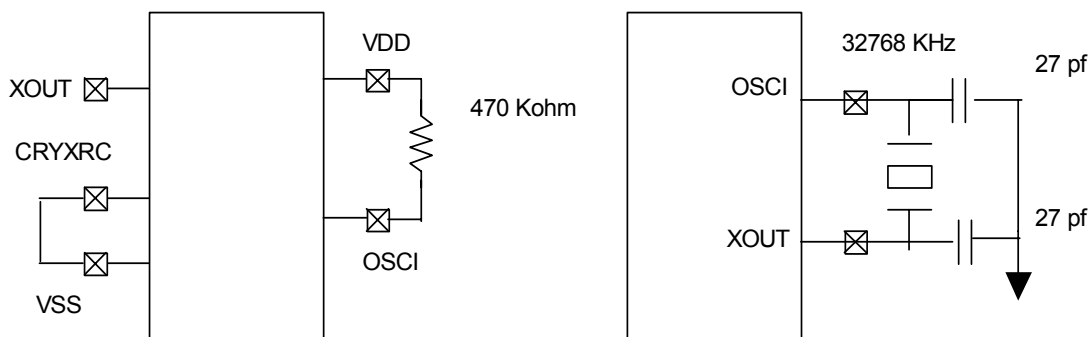
Fig. 15 RC/Crystal OSC Block Diagram
