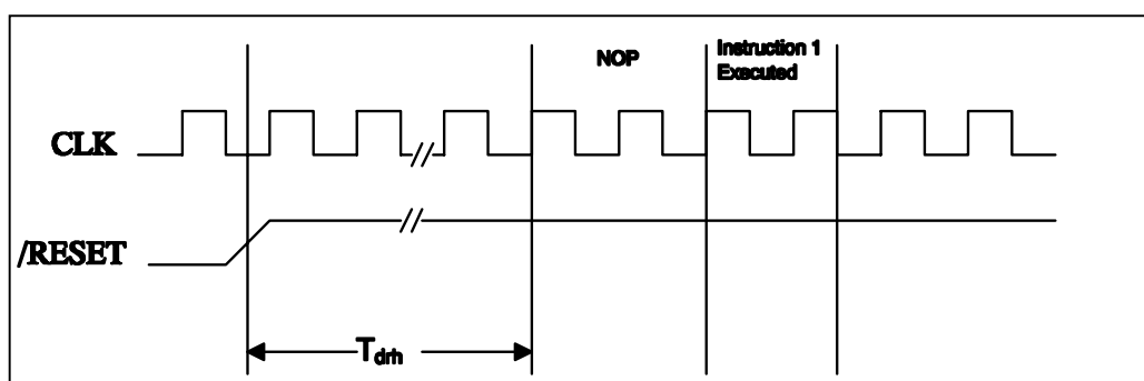
Fig. 17b RESET Timing Diagram
