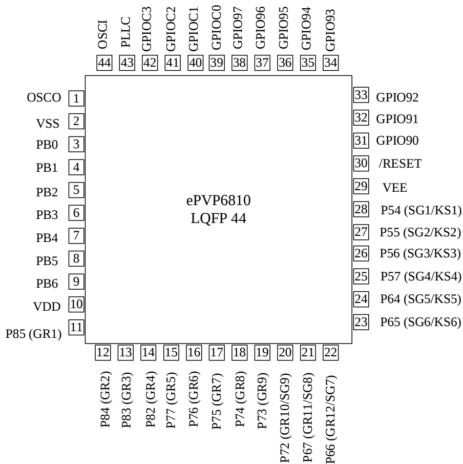
Fig. 1 Pin Assignment
