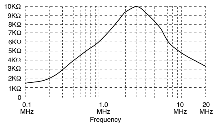
Impedance Curve
