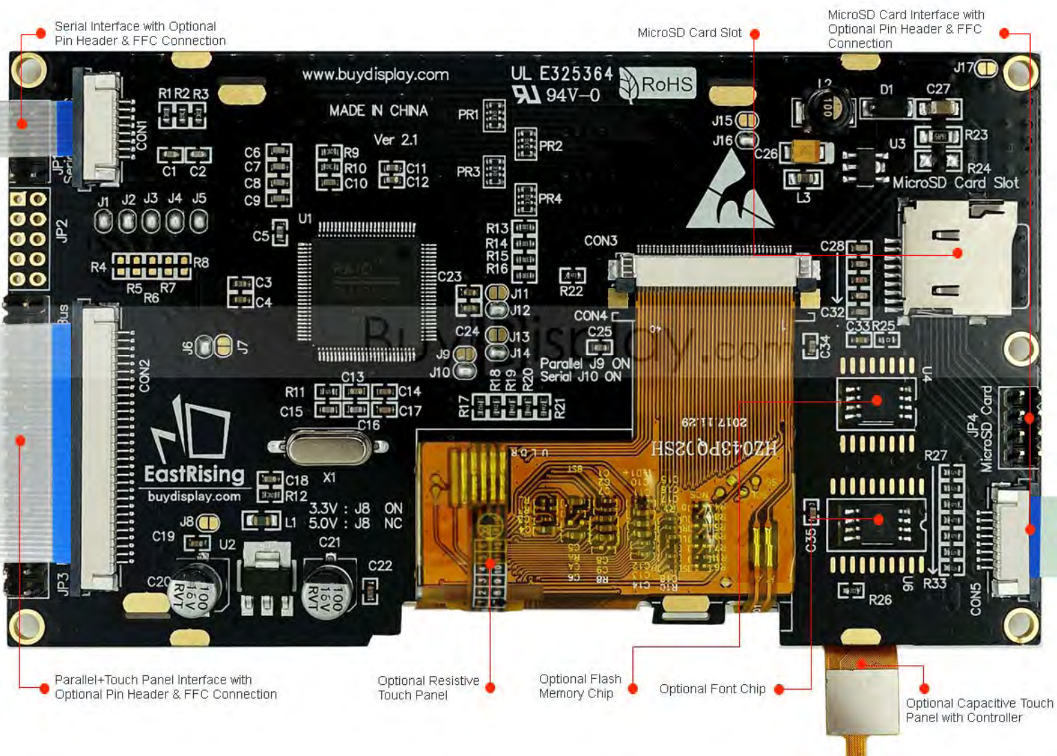
ER-TFTM043-3 Controller Board with Optional Capacitive & Resistive Touch Panel
