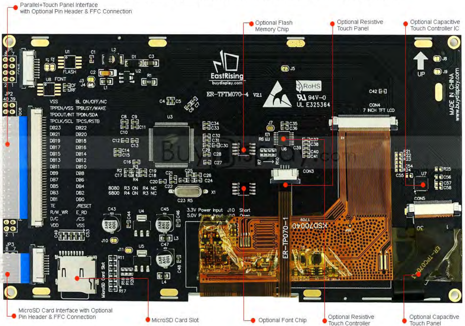
ER-TFTM070-4V2.1 with Optional Capacitive & Resistive Touch Panel
