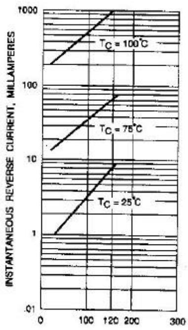
Fig. 3-TYPICAL REVERSE CHARACTERISTICS
