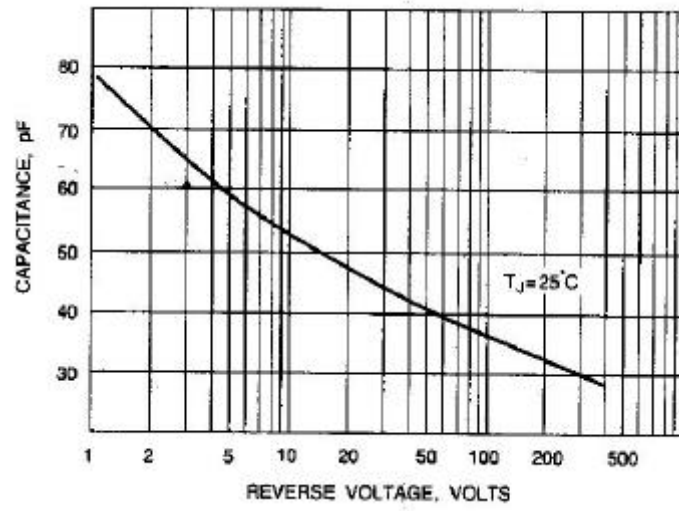
Fig. 5-TYPICAL JUNCTION CAPACITANCE
