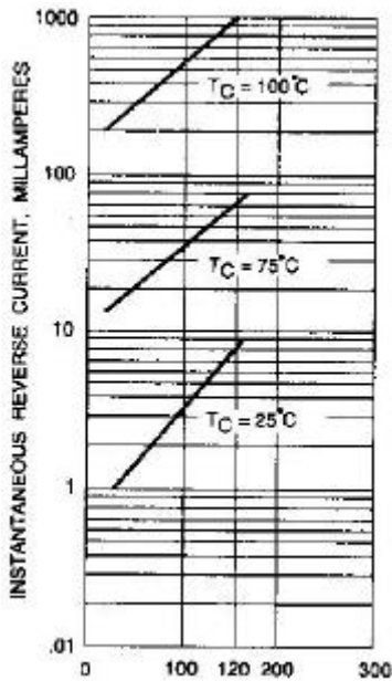
Fig. 3-TYPICAL REVERSE CHARACTERISTICS
