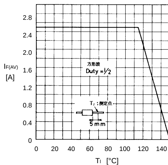
Current derating ( I_{F(AV)}-T_i )
