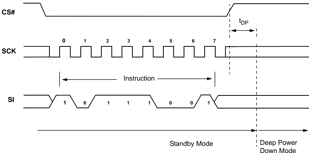
Figure 16. Deep Power Down ( DP ) Instruction Sequence
