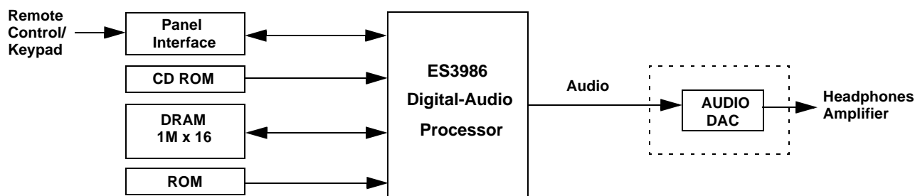
Figure 1 ES3986 VCD Processor System Block Diagram
