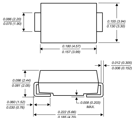
Case: SMB Dimensions in inches and (millimetres)
