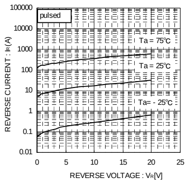
Fig.1 Reverse Current vs. Reverse Voltage
