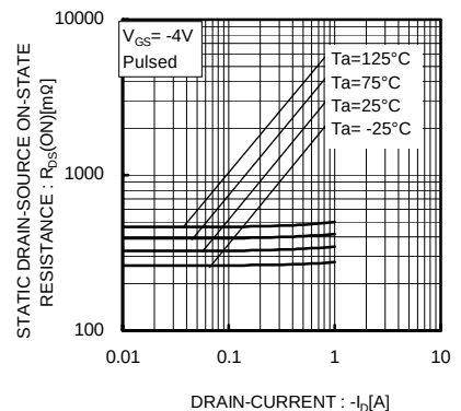
Fig.6 Static Drain-Source On-State Resistance vs. Drain Current(III)
