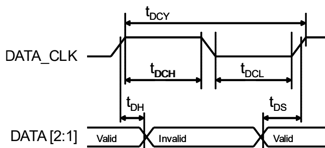
Figure 25 - Audio Interface Timing
