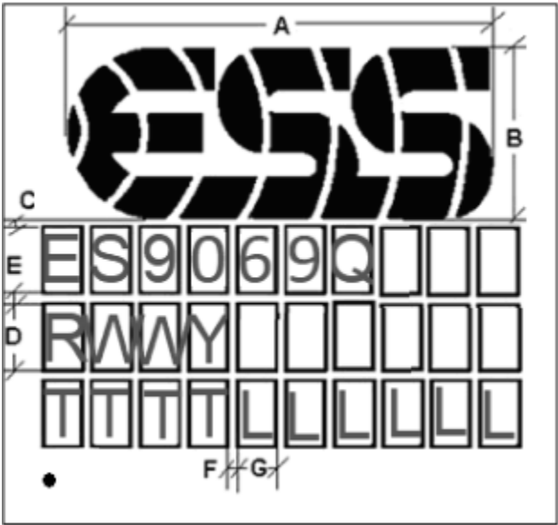
Figure 31 - ES9069Q Marking
