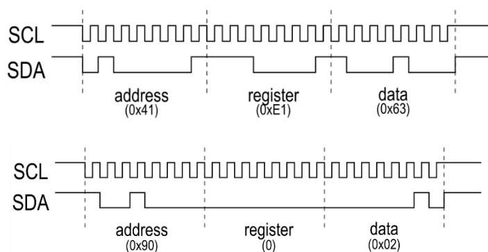
Figure 21 - I 2 C Single Byte Examples of Read and Write Instructions
