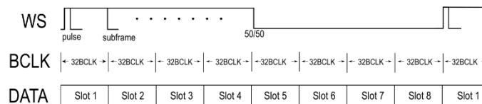
Figure 9 - TDM256 Mode
