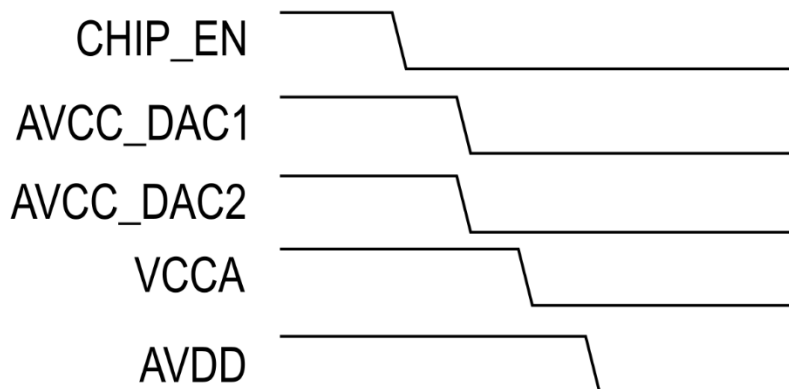
Figure 19 – Recommended Power Down Sequence
