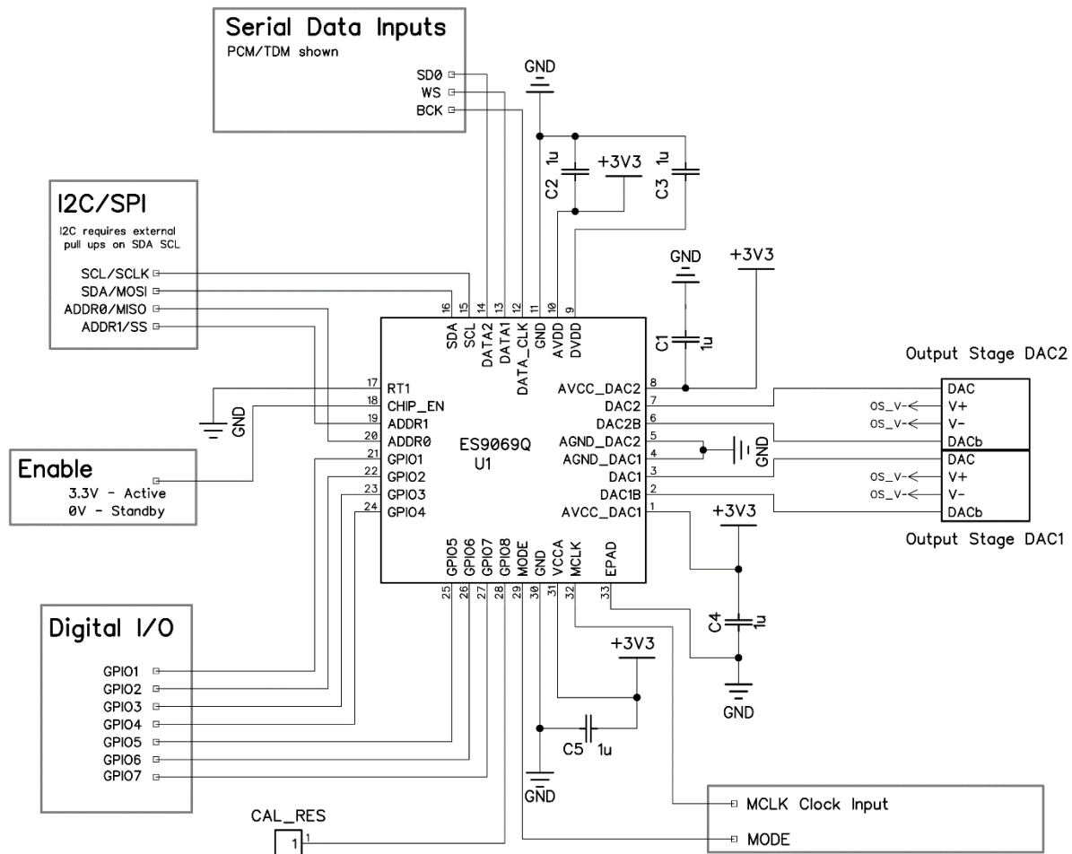
Figure 28 - Software Mode Reference Schematic for ES9069
