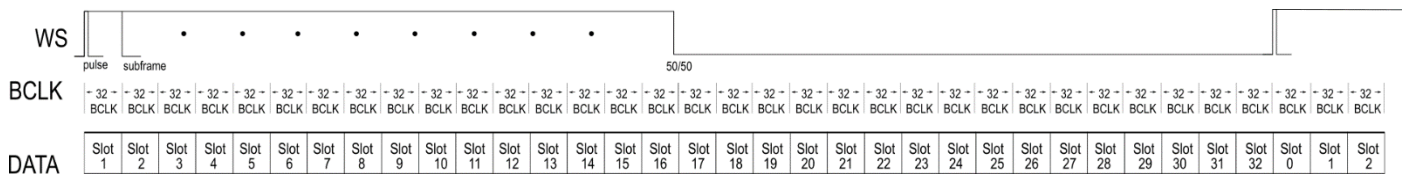
Figure 11 - TDM1024 Mode
