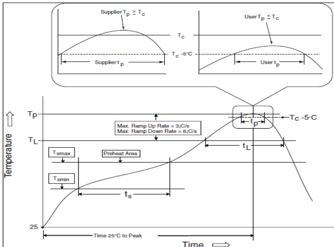
Figure 32 - IR/Convection Reflow Profile (IPC/JEDEC J-STD-020D.1)
