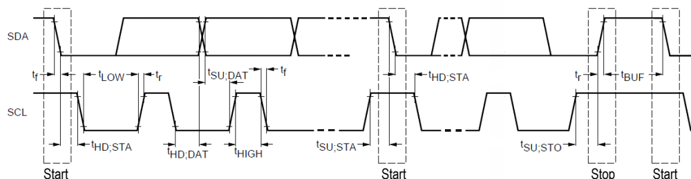
Figure 20 - I 2 C Slave Control Interface Timing
