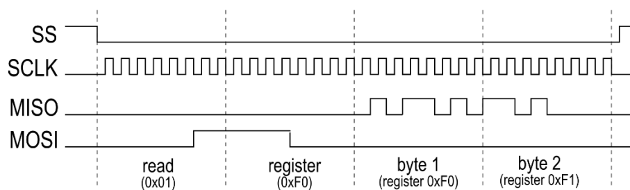
Figure 24 - SPI Multi-Byte Read
