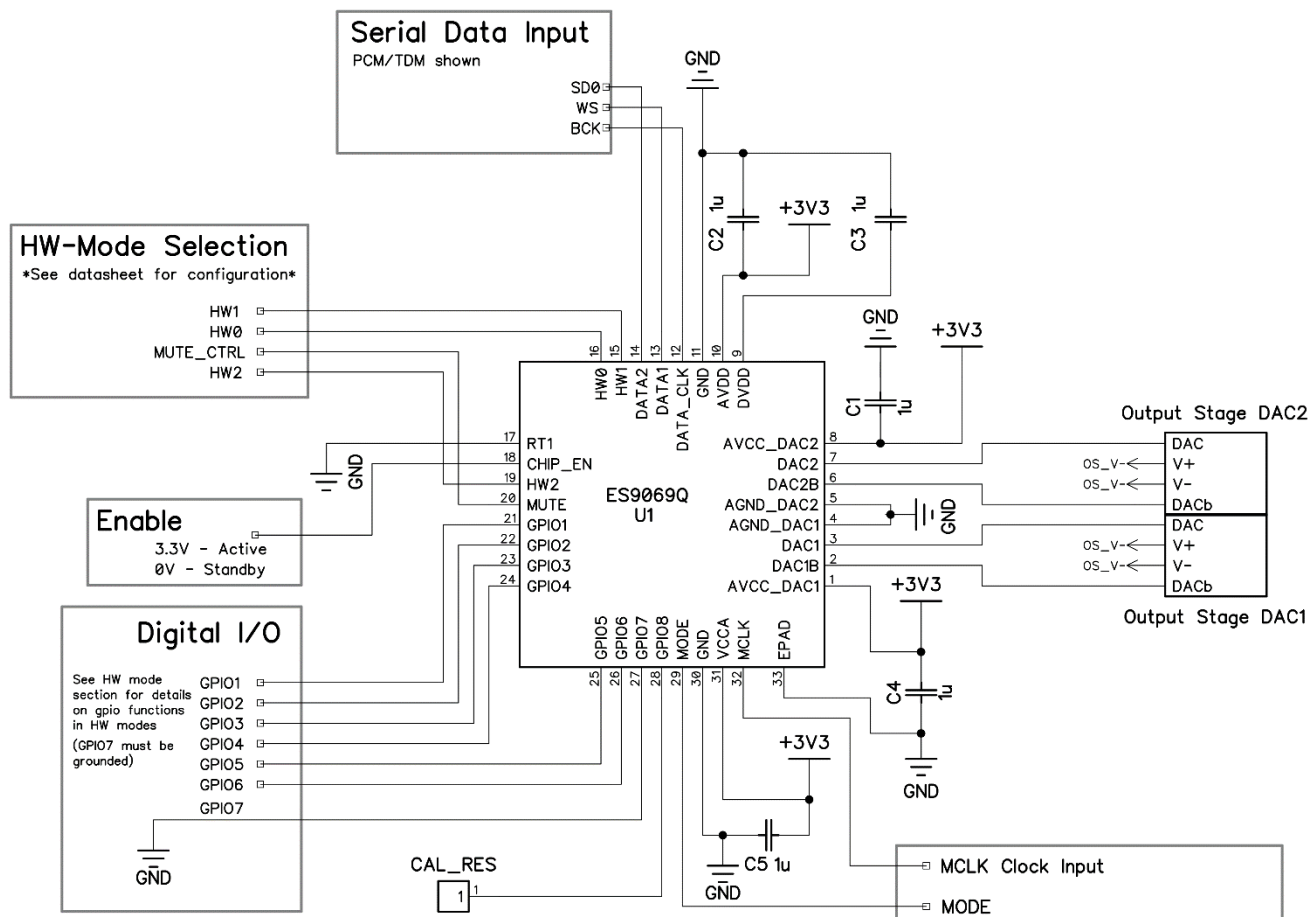
Figure 27 - Hardware (HW) Mode Reference Schematic for ES9069
