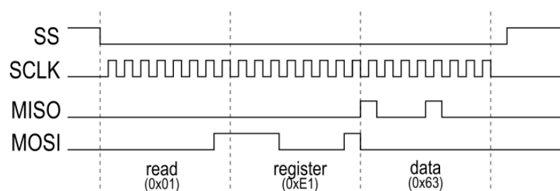
Figure 23 - SPI Single Byte Read
