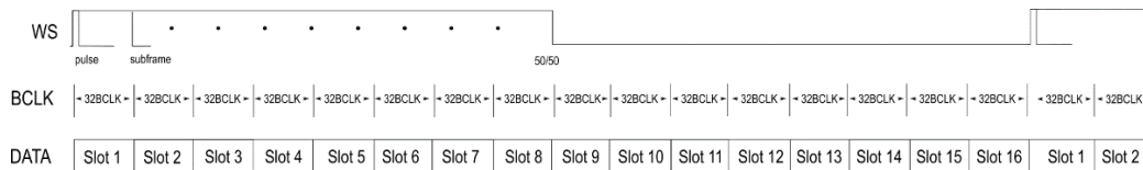
Figure 10 - TDM512 Mode
