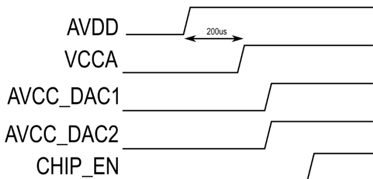
Figure 18 – Recommended Power Up Sequence
