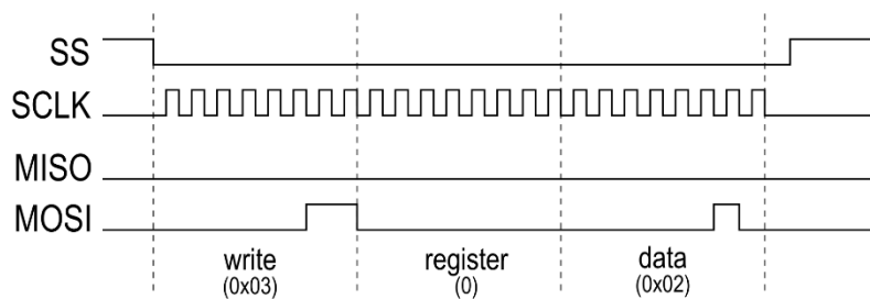
Figure 22 - SPI Single Byte Write
