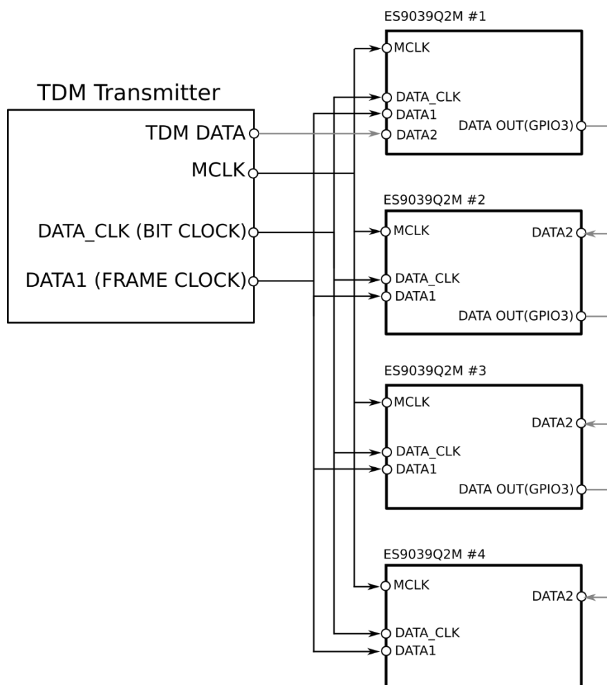
Figure 13 - TDM Connection of Several ES9069 Devices in Daisy Chain Mode
