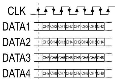
Figure 17 - PDM 8 Channel Format
