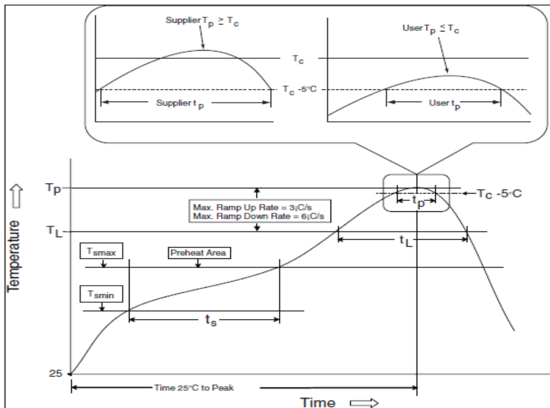
Figure 38 - IR/Convection Reflow Profile (IPC/JEDEC J-STD-020D.1)
