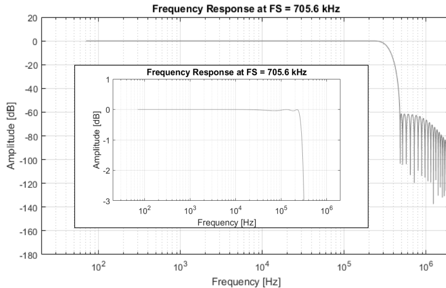
Figure 21 - Minimum Phase 64FS Frequency Response
