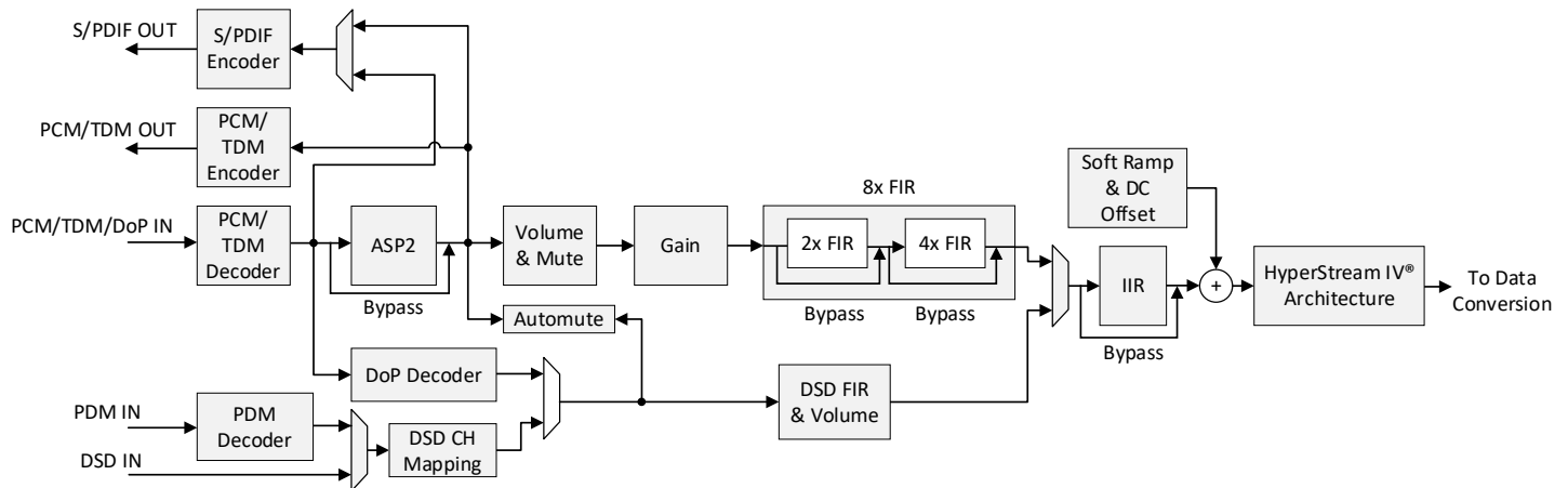
Figure 18 - Digital Signal Path
