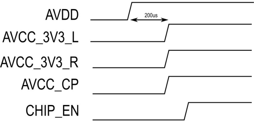
Figure 29 - Recommended Power Up Sequence
