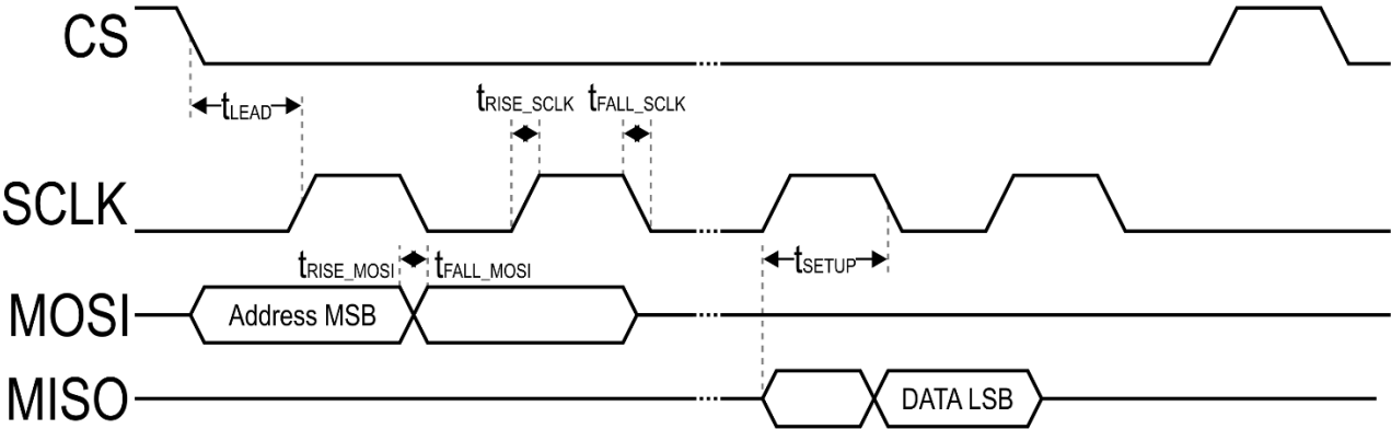
Figure 28 - SPI Master Interface Timing
