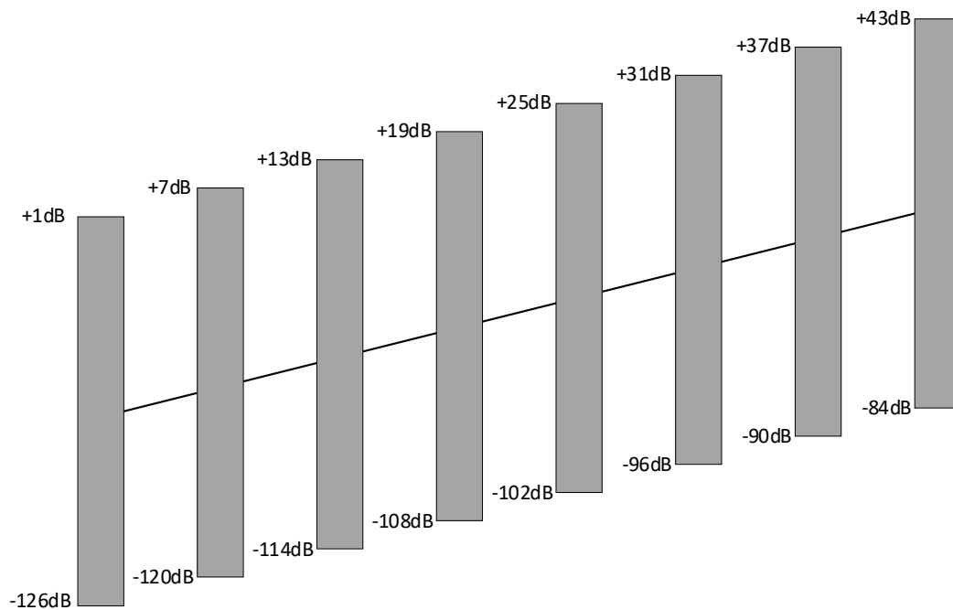
Figure 20 - ES9082 Volume and Gain Range
