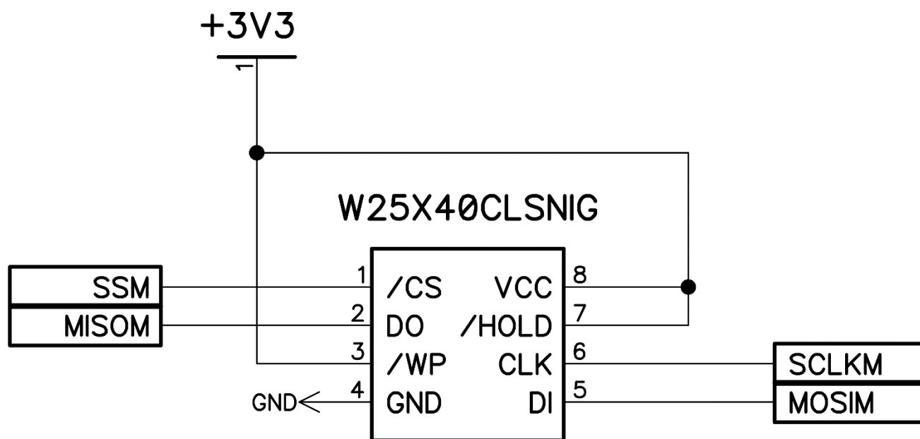
Figure 34 - Example SPI Flash Schematic
