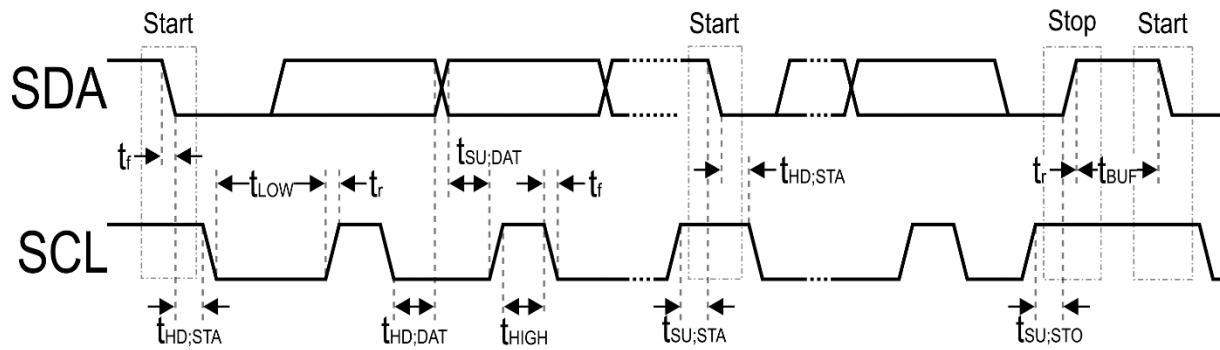
Figure 26 - I 2 C Slave Control Interface Timing
