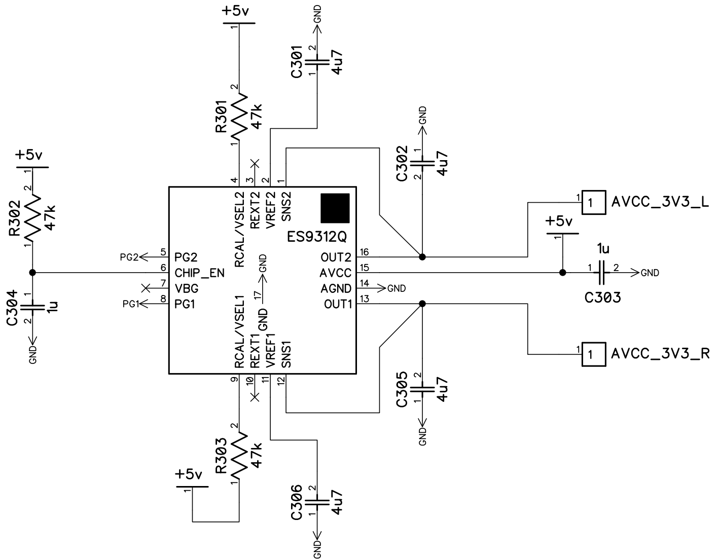
Figure 33 - ES9082 Power Supply Schematic
