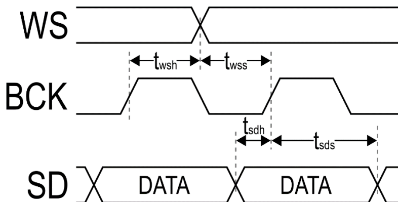
Figure 25 - Bit-Clock and Word-Select Timing
