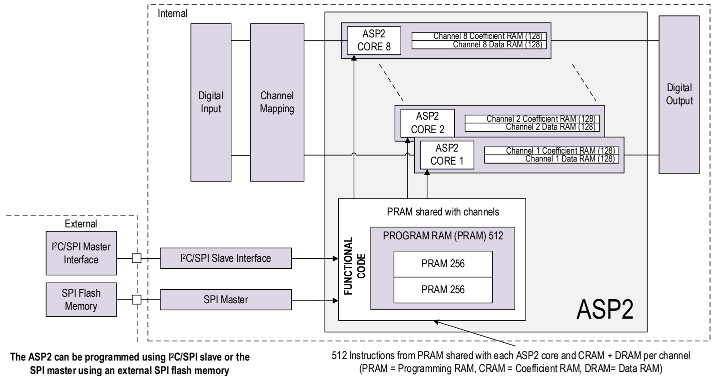
Figure 19 - Top level view of ES9082 ASP2
