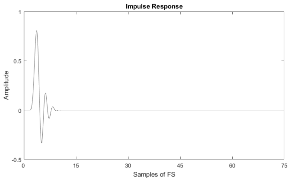
Figure 22 - Minimum Phase 64FS Impulse Response
