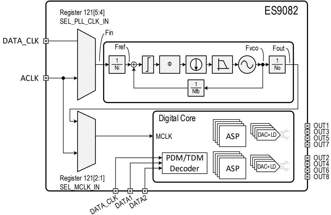
Figure 24 - Functional Block Diagram of ES9082 APLL
