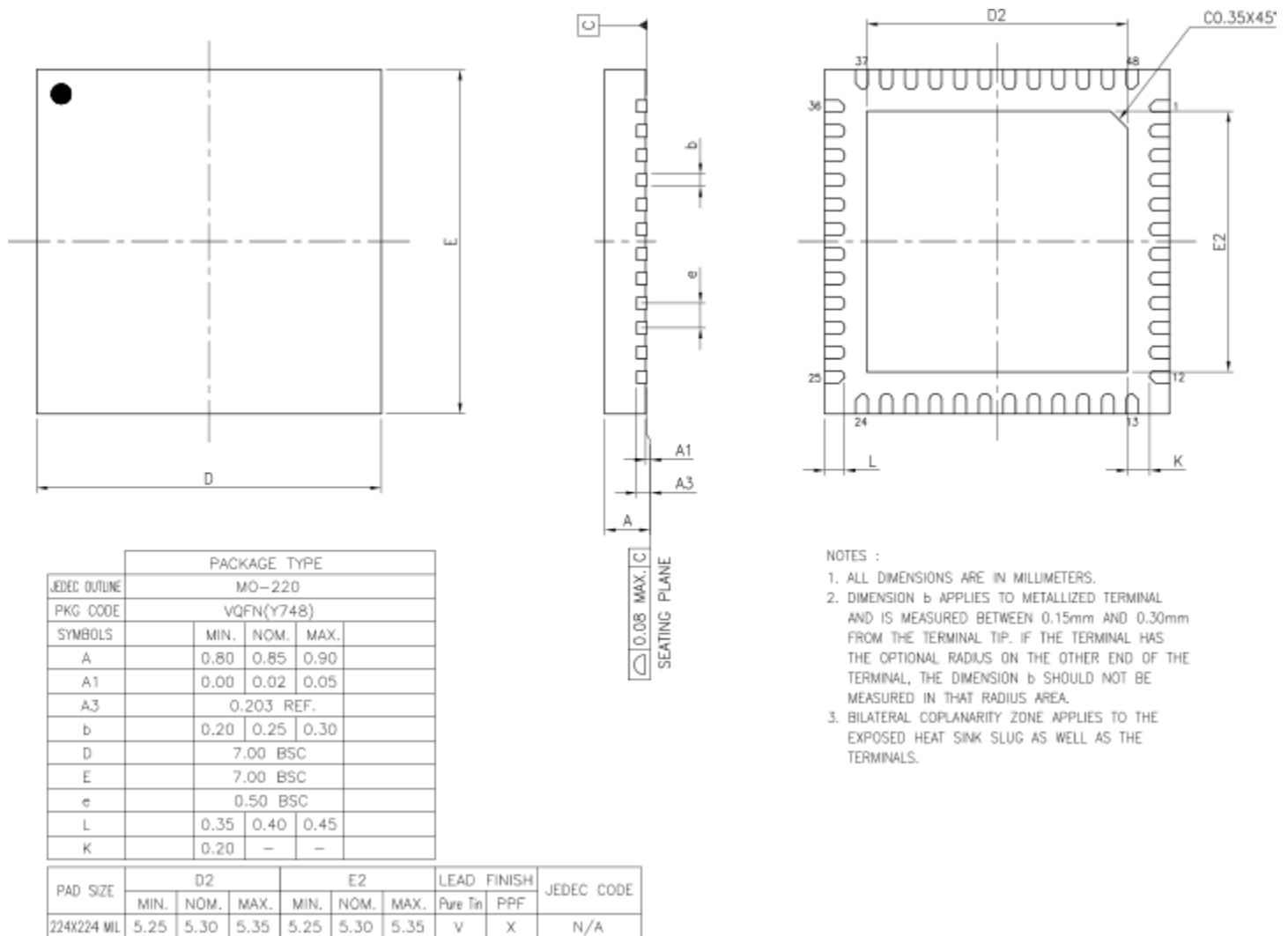
Figure 36 – ES9082 48 QFN Package Dimensions
