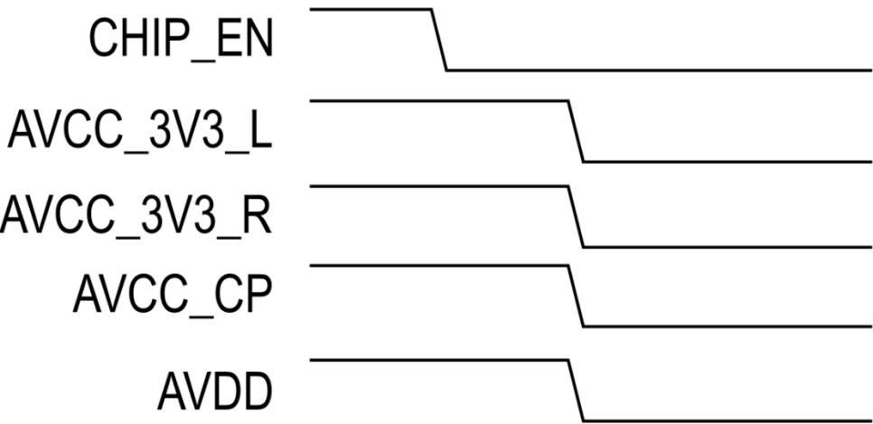
Figure 30 - Recommended Power Down Sequence
