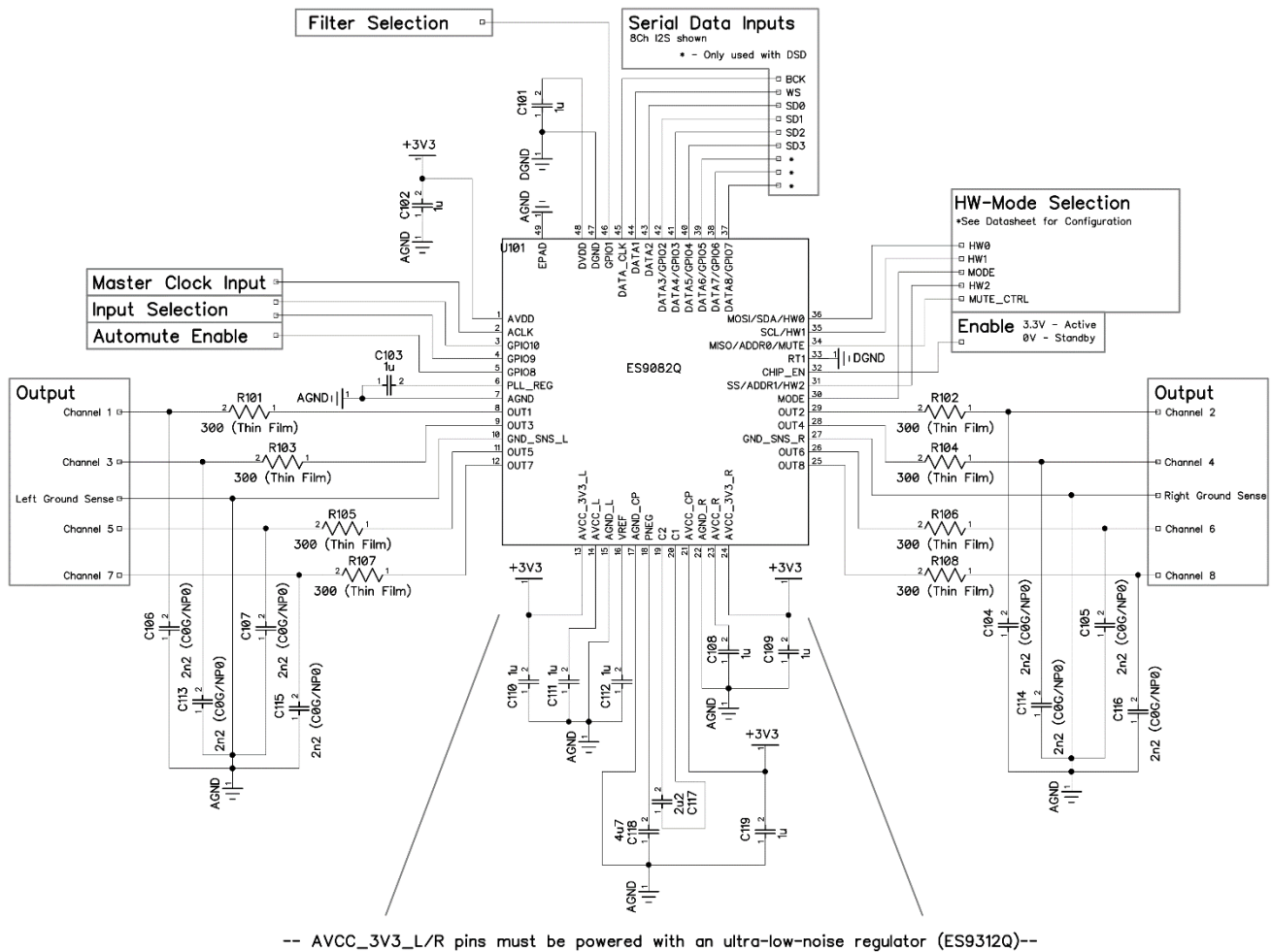
Figure 31 - ES9082 Hardware Mode Reference Schematic
