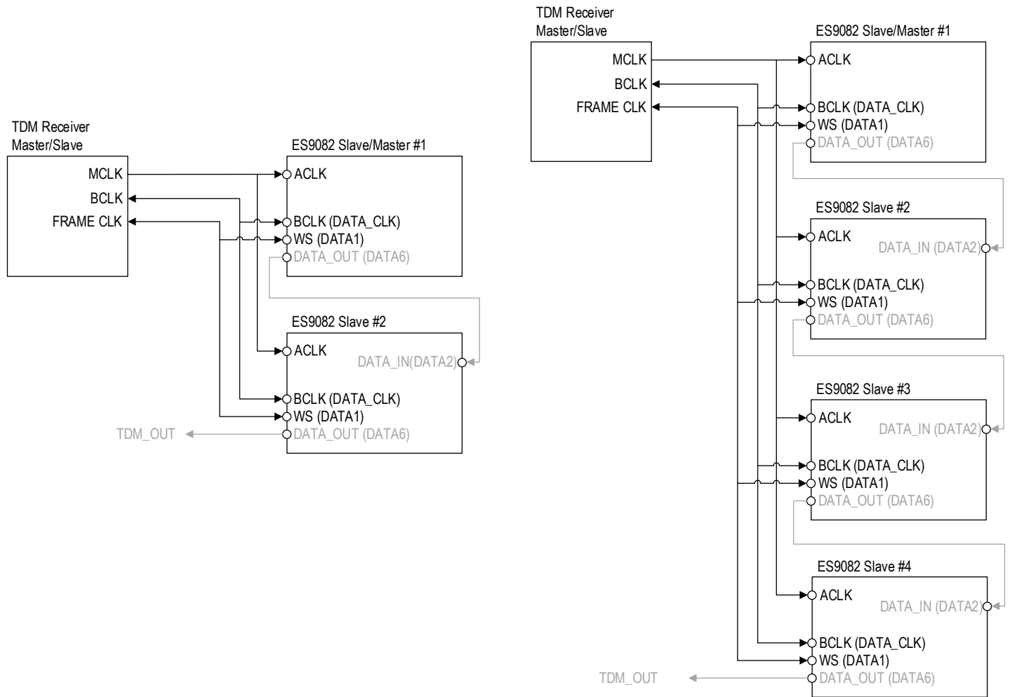
Figure 23 - Example Connection for TDM Decoder Daisy Chain Mode
