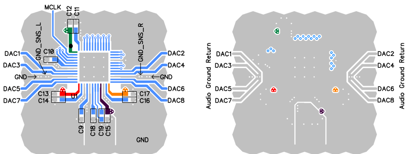
Figure 35 - ES9082 Recommended PCB Layout Guidelines
