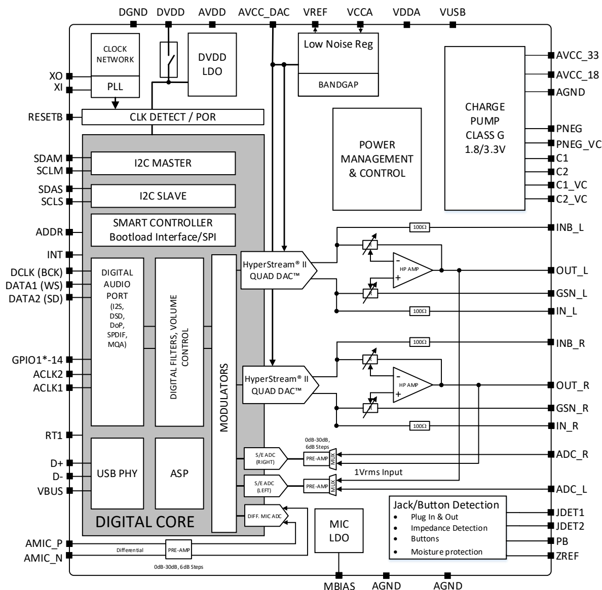
Figure 2 – ES9281A/80A PRO Block Diagram
