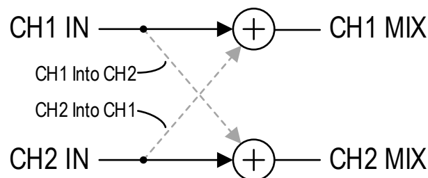
Figure 18 - DAC Mixing
