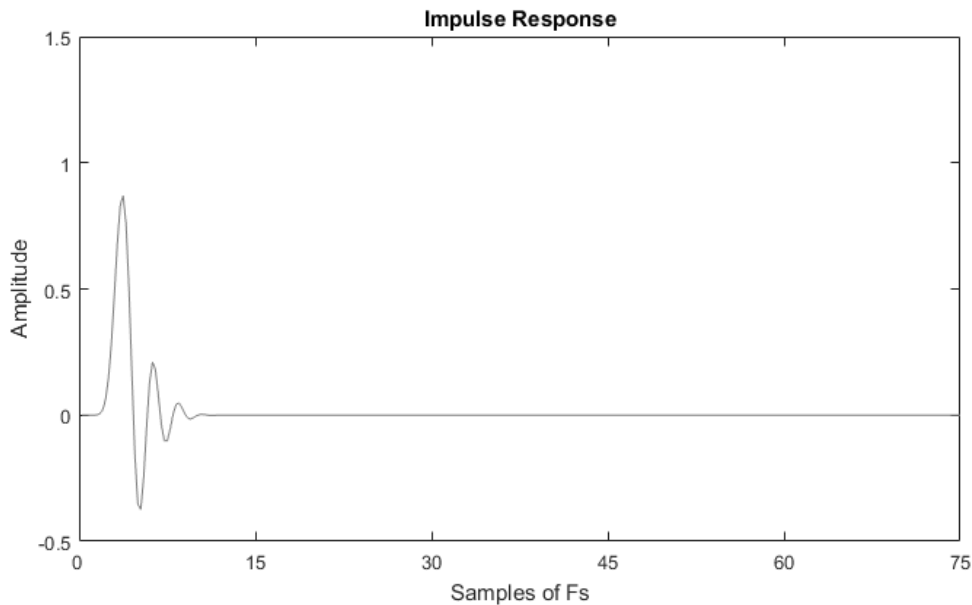
Figure 20 - ADC Minimum Phase 64FS Impulse Response
