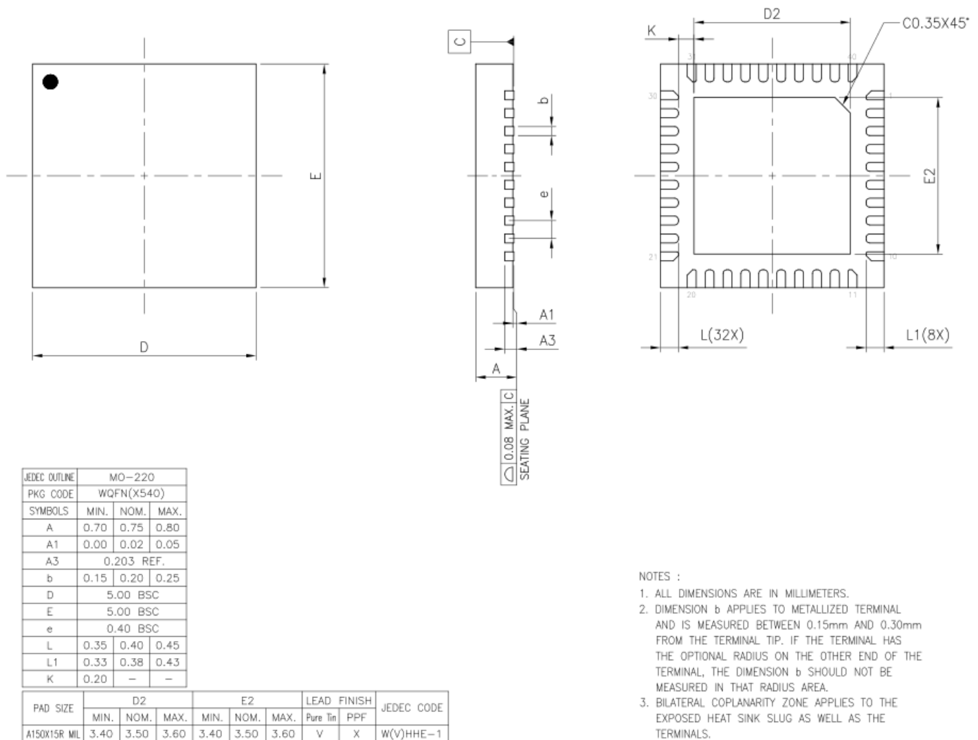
Figure 31 - ES9290 40 QFN Package Dimensions
