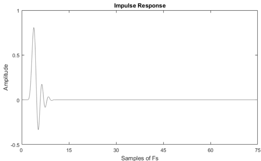
Figure 22 - DAC Minimum Phase 64FS Impulse Response
