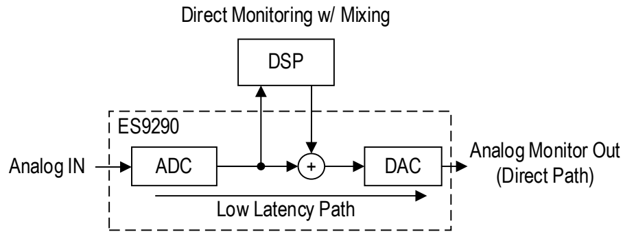
Figure 10 - Direct Monitoring Path
