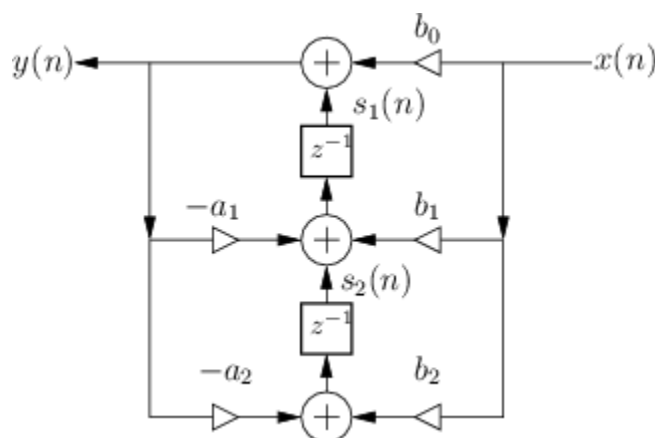
Figure 34 - Direct-Form Transposed II BiQuad
