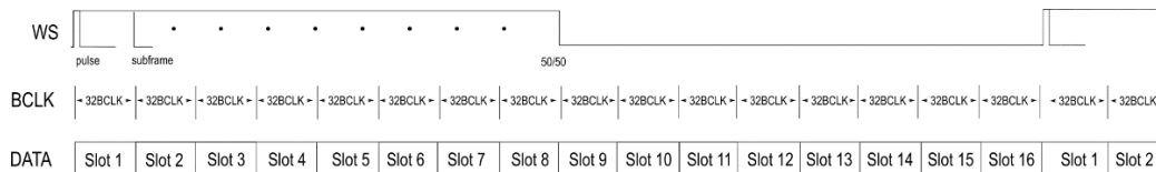
Figure 14 - TDM16 Mode
