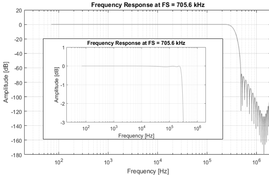
Figure 19 - ADC Minimum Phase 64FS Frequency Response
