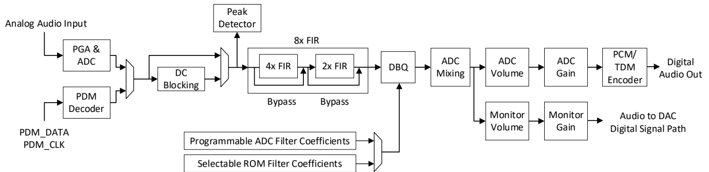
Figure 16 - ADC Digital Signal Path
