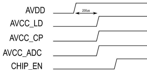
Figure 27 - Recommended Power Up Sequence
