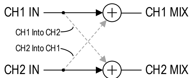
Figure 17 - ADC Mixing
