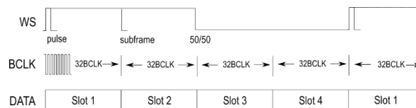
Figure 12 - TDM4 Mode
