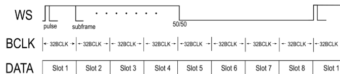
Figure 13 - TDM8 Mode
