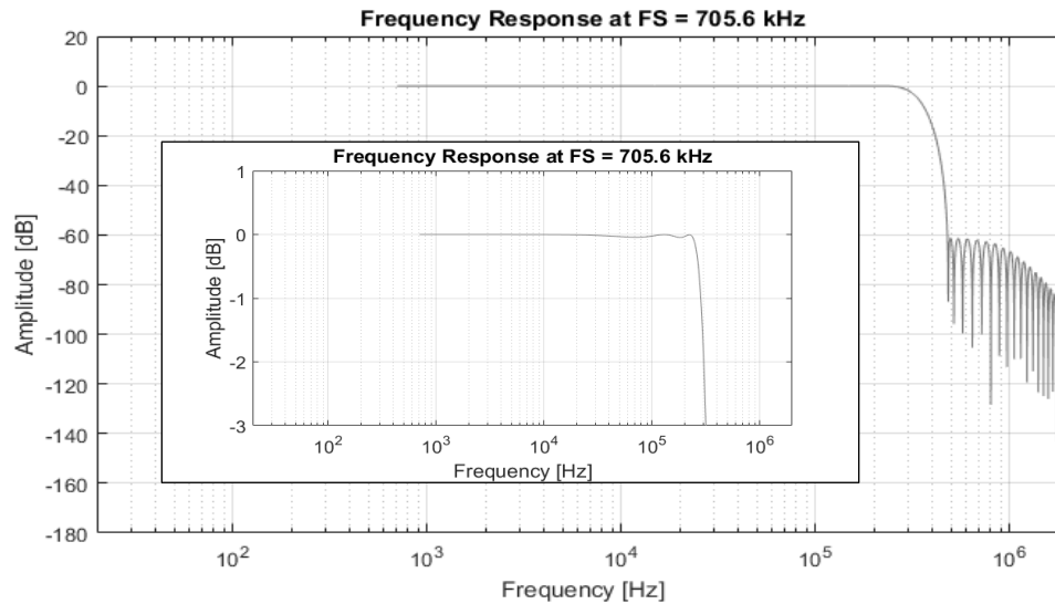
Figure 21 - DAC Minimum Phase 64FS Frequency Response
