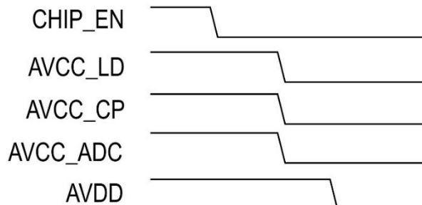
Figure 28 - Recommended Power Down Sequence
