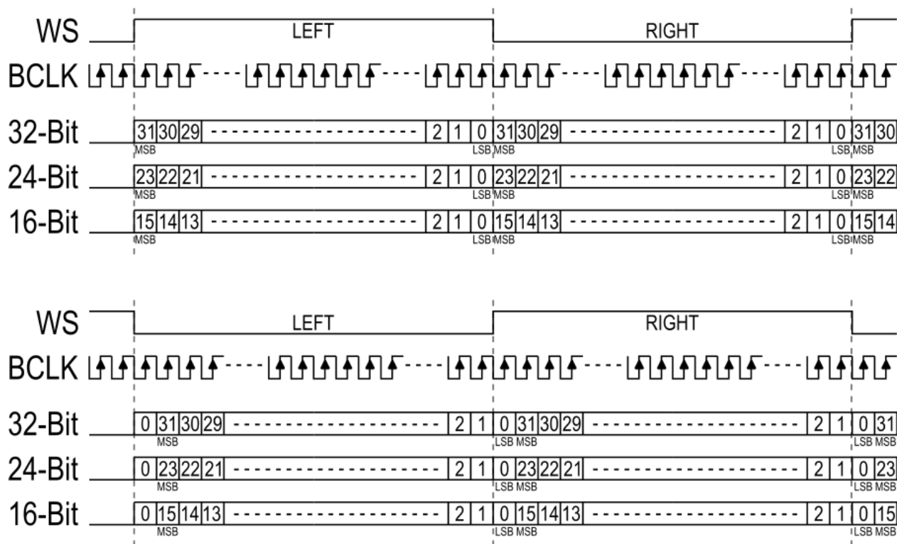
Figure 11 - LJ (top) & I 2 S (bottom) for 32, 24, and 16-bit Word Widths
