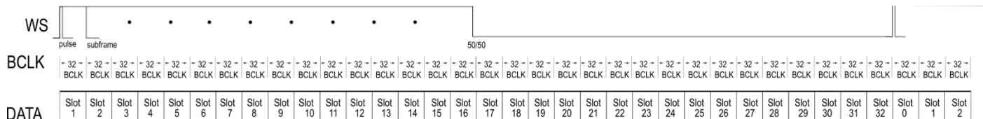
Figure 15 - TDM32 Mode
