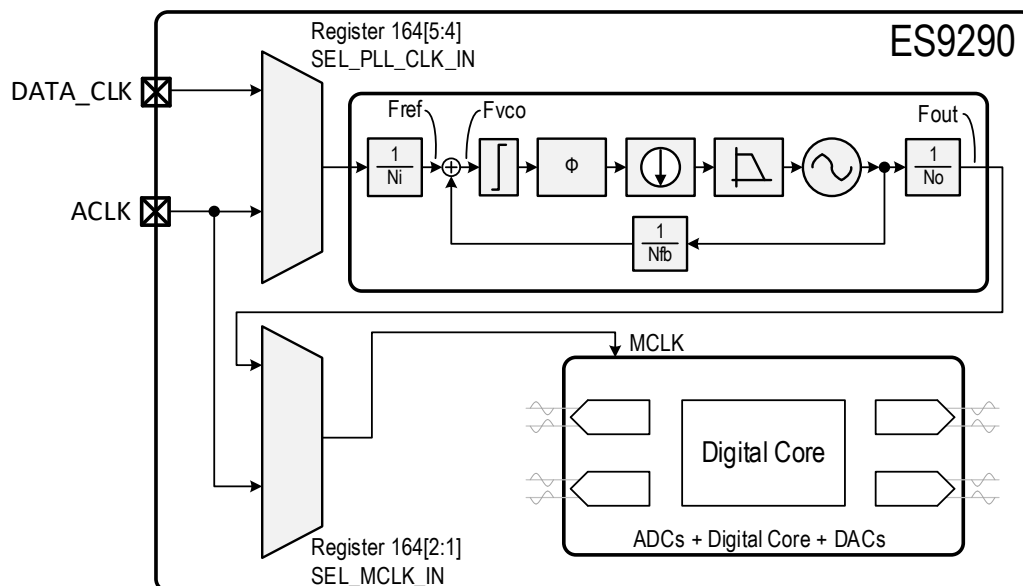
Figure 24 - Functional Block Diagram of ES9290 APLL
