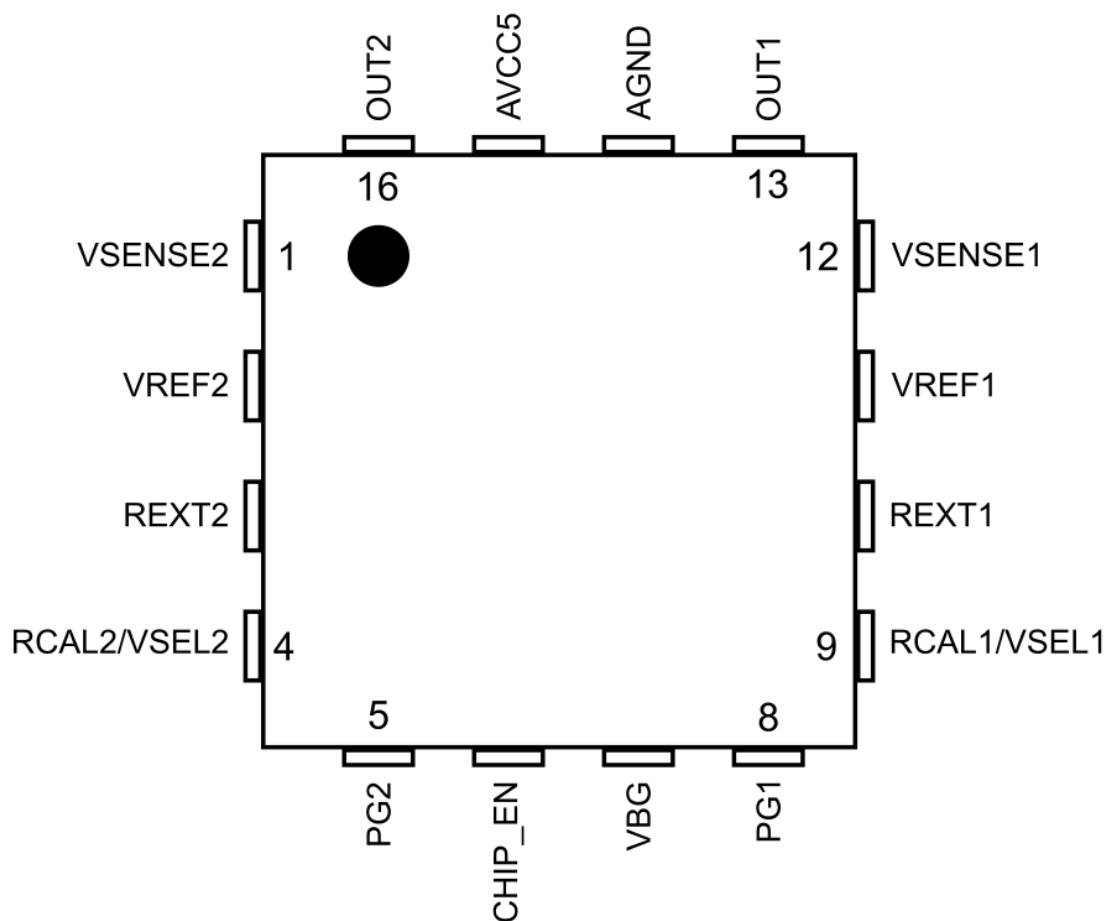
Figure 1 - 16 QFN Pinout
