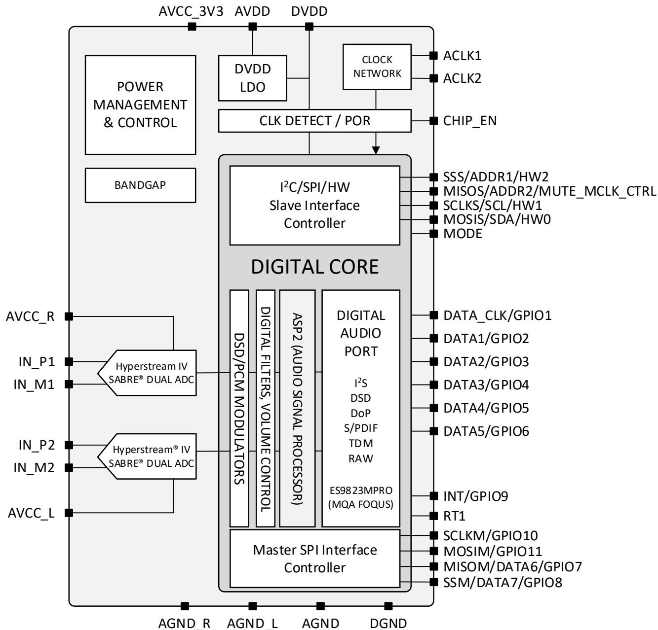
Figure 1 - ES9823MPRO &amp; ES9823PRO Block Diagram
