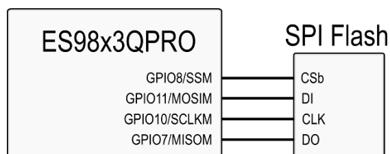
Figure 13 - Example SPI Flash Schematic
