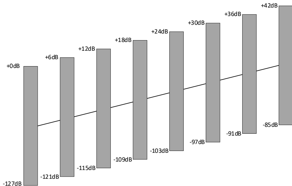
Figure 17 - ES9823MPRO & ES9823PRO Volume and Gain Range
