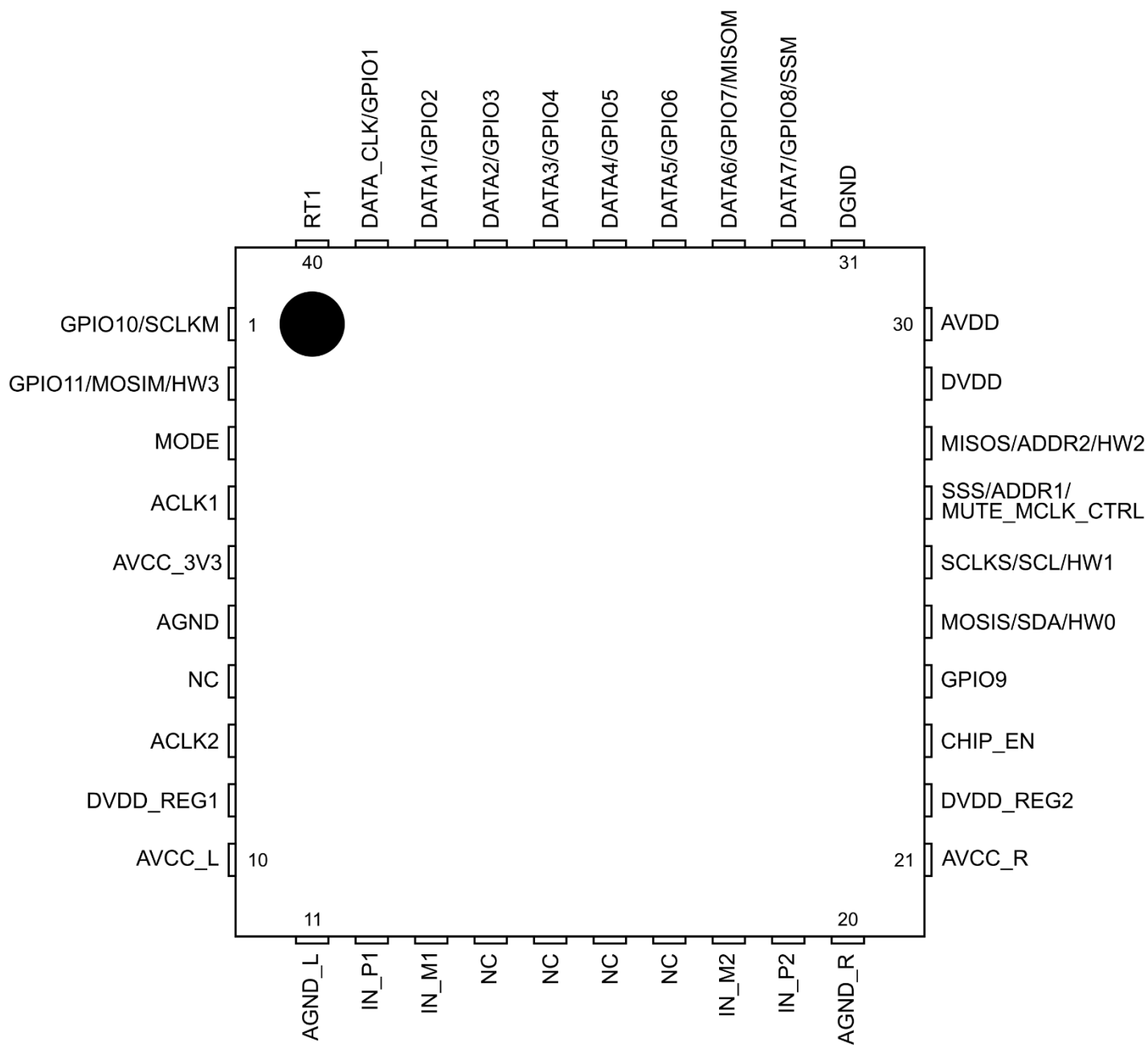
ES9823QPRO (Top View)
