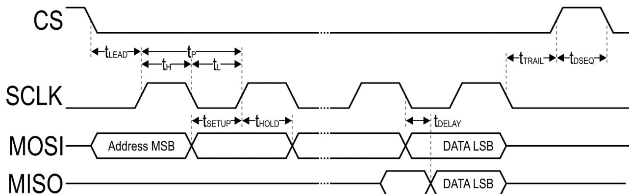
Figure 25 - SPI Slave Interface Timing
