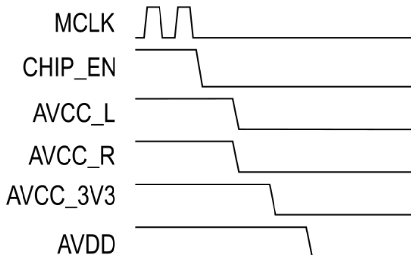
Figure 27 - Recommended Power Down Sequence
