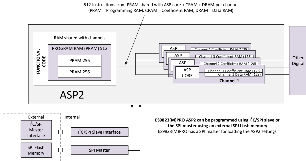
Figure 16 - Top Level View of ES9823MPRO & ES9823PRO ASP2
