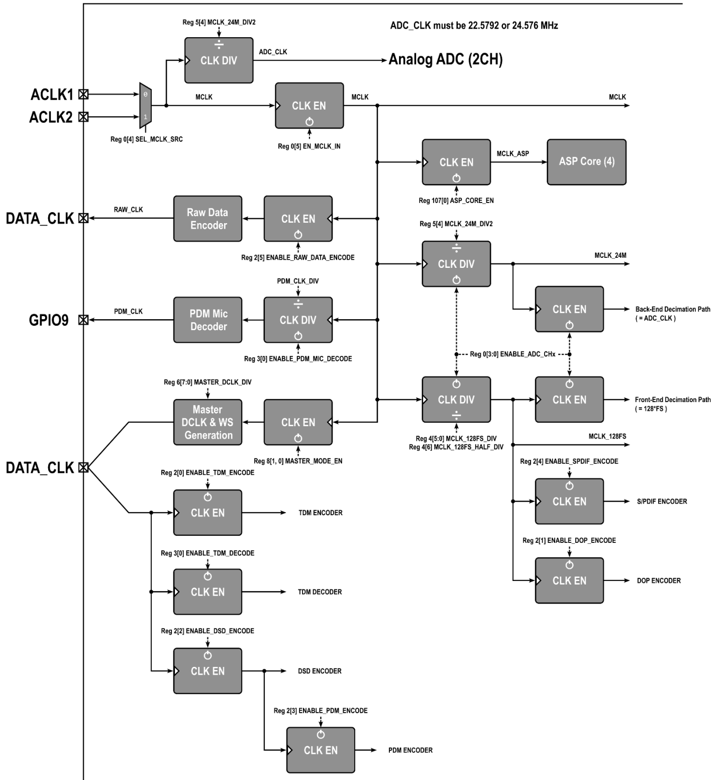
Figure 21 - Clock Distribution
