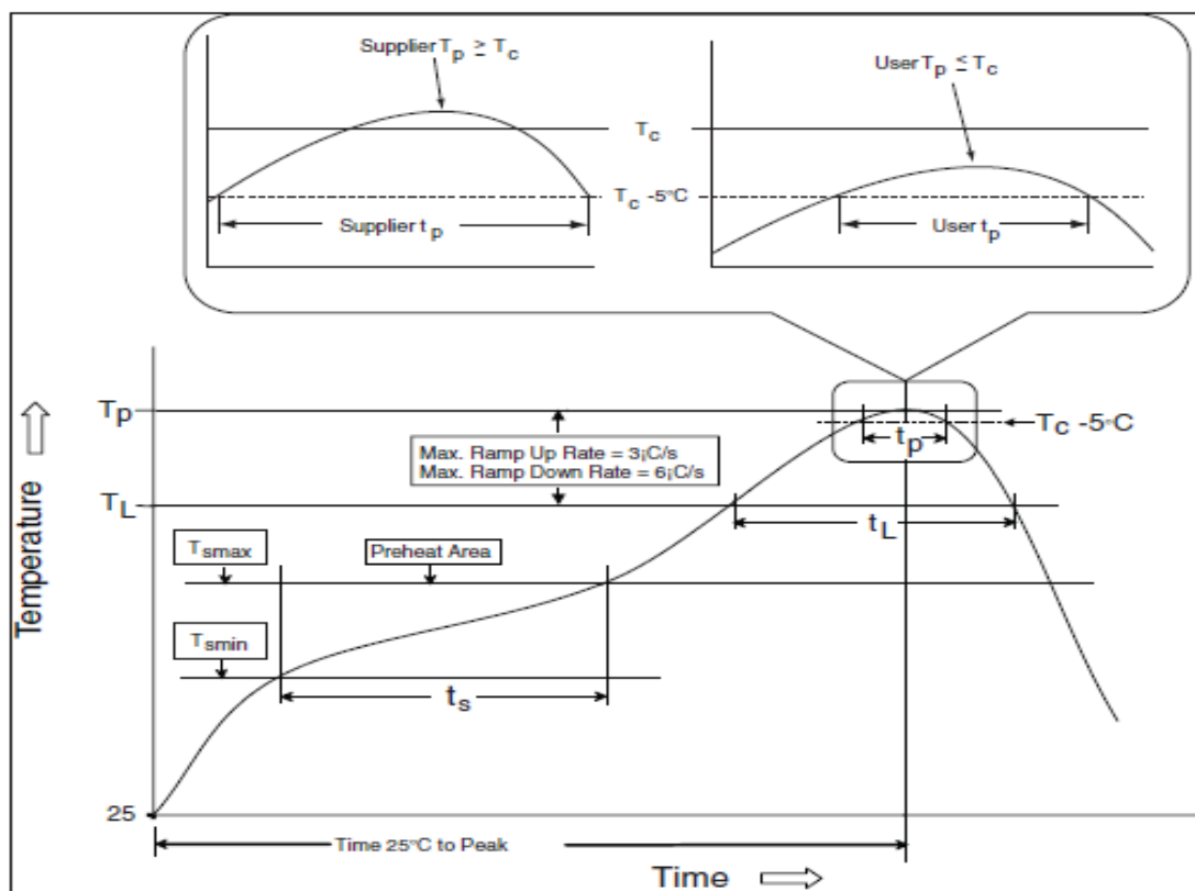
Figure 37 - IR/Convection Reflow Profile (IPC/JEDEC J-STD-020D.1)
