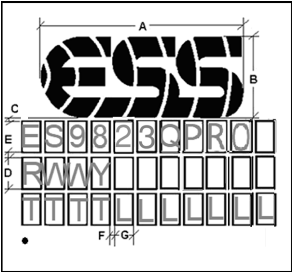
Figure 35 - ES9823QPRO Top View Marking
