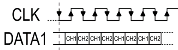
Figure 12 - PDM 2 Channel Format
