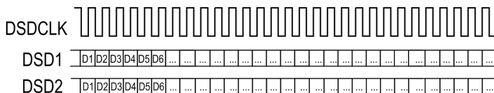
Figure 11 - DSD Format, 1-bit stream
