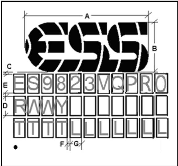
Figure 36 - ES9823MQPRO Top View Marking
