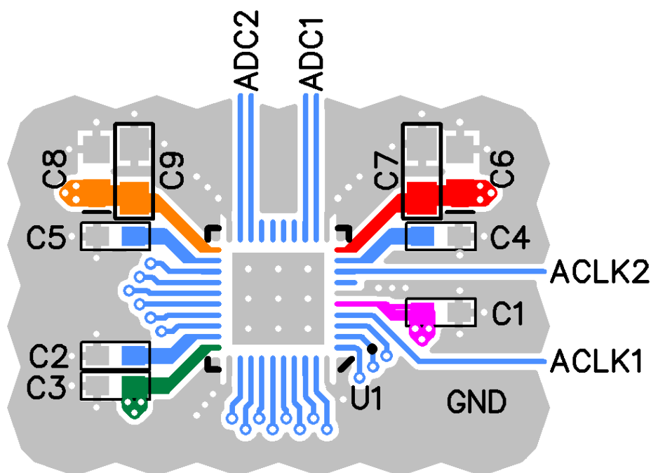
Figure 33 - ES9823MPRO & ES9823PRO Recommended PCB Layout Guidelines
