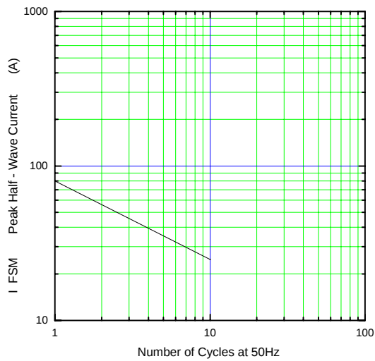
Surge Capability
