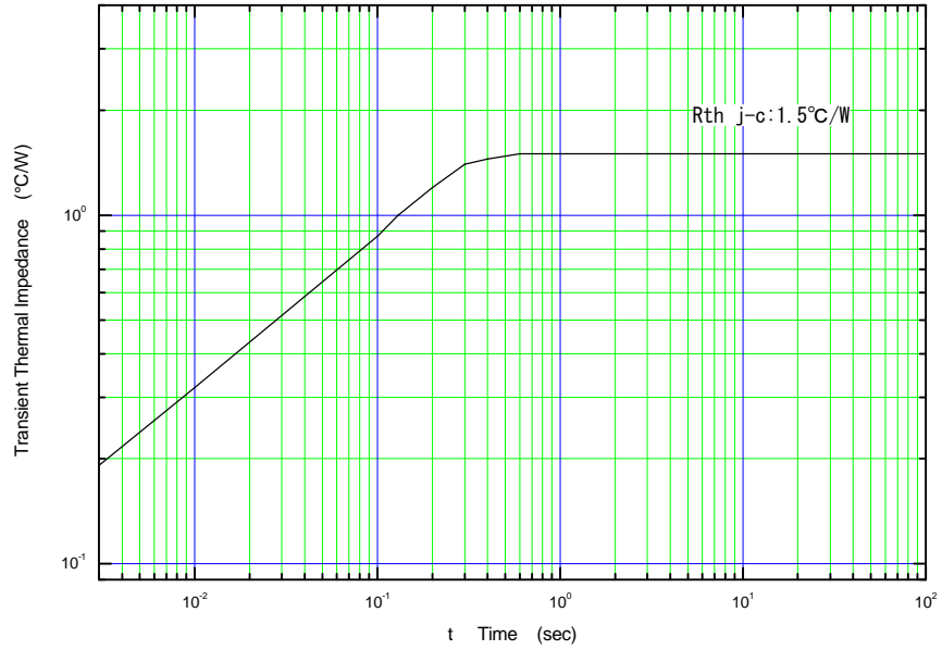
Transient Thermal Impedance (max.)
