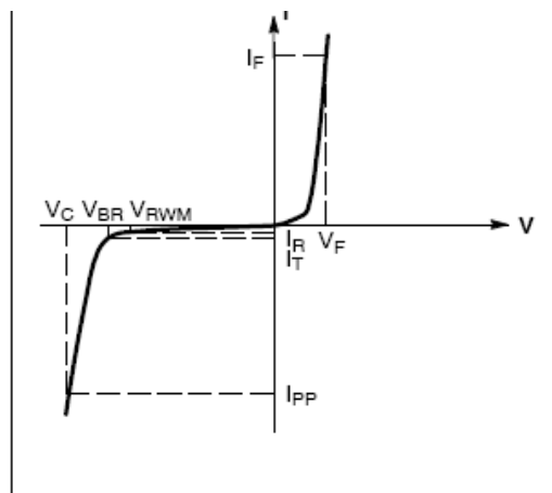
Figure 1. Uni-Directional TVS
