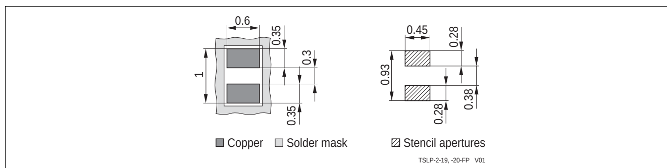
Figure 6-6 TSLP-2-20: Footprint
