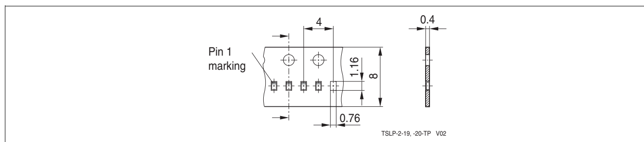
Figure 6-7 TSLP-2-20: Packing
