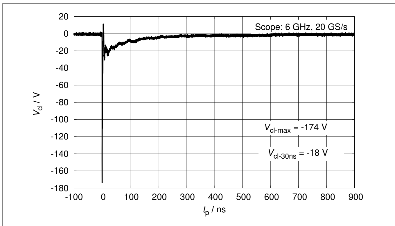
Figure 8 Clamping voltage (ESD): V_{cl} = f(t_p) , 15 kV negative pulse according to IEC61000-4-2
