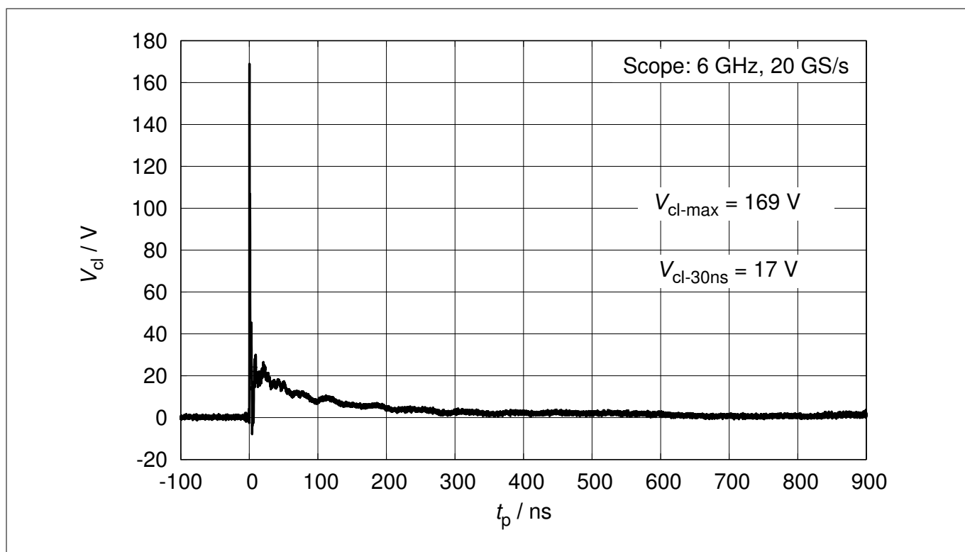
Figure 7 Clamping voltage (ESD): V_{cl} = f(t_p) , 15 kV positive pulse according to IEC61000-4-2
