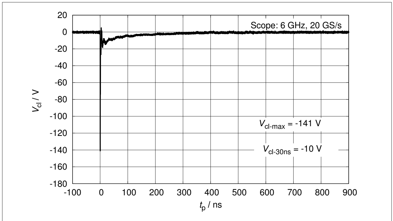
Figure 6 Clamping voltage (ESD): V_{cl} = f(t_p) , 8 kV negative pulse according to IEC61000-4-2
