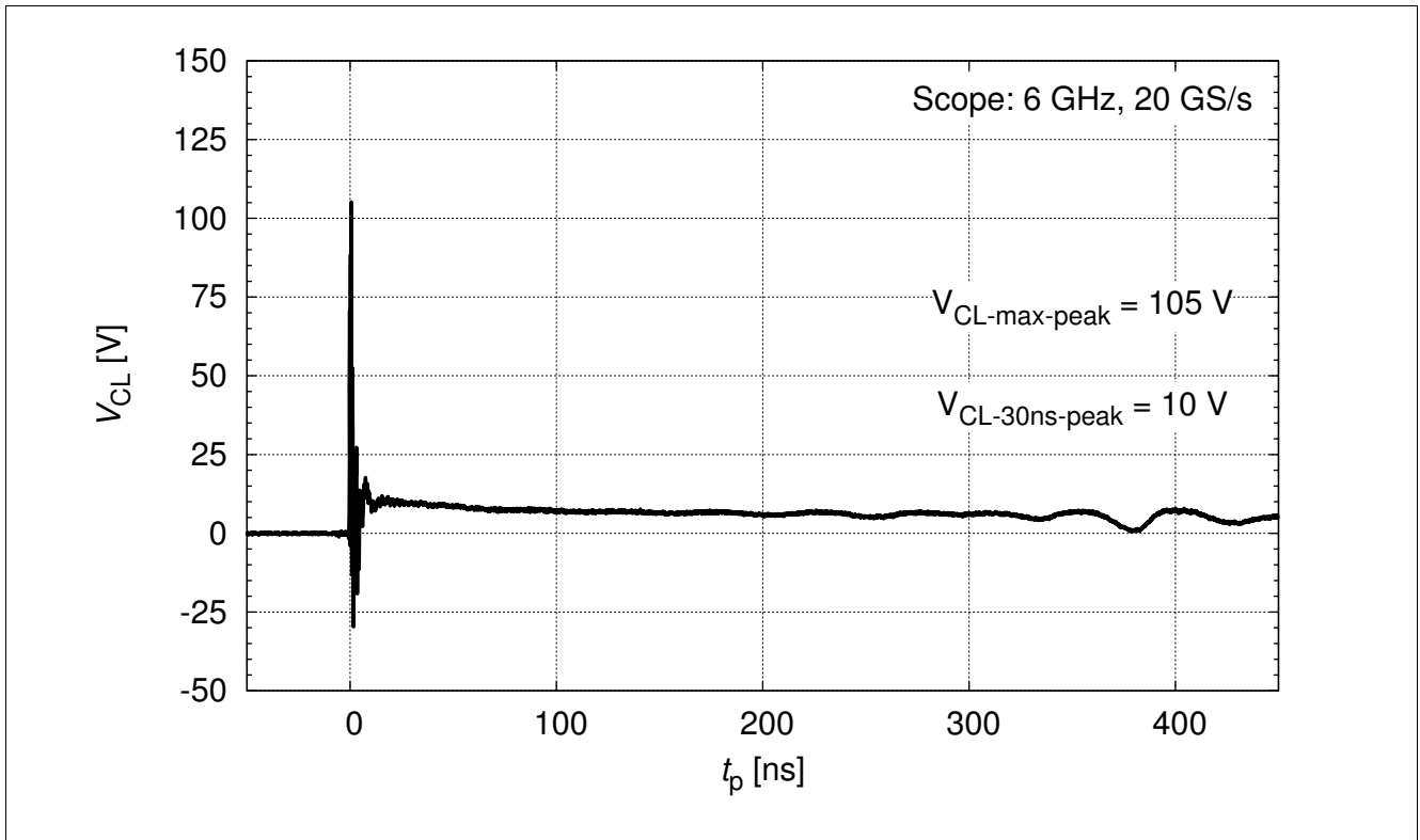
Figure 3-7 Clamping voltage at +15 kV discharge according IEC61000-4-2 ( R = 330\text{ } \Omega , C = 150\text{ pF} )
