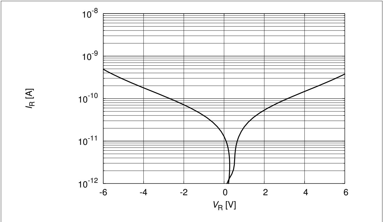
Figure 3-1 Reverse current, I_R = (V_R)
