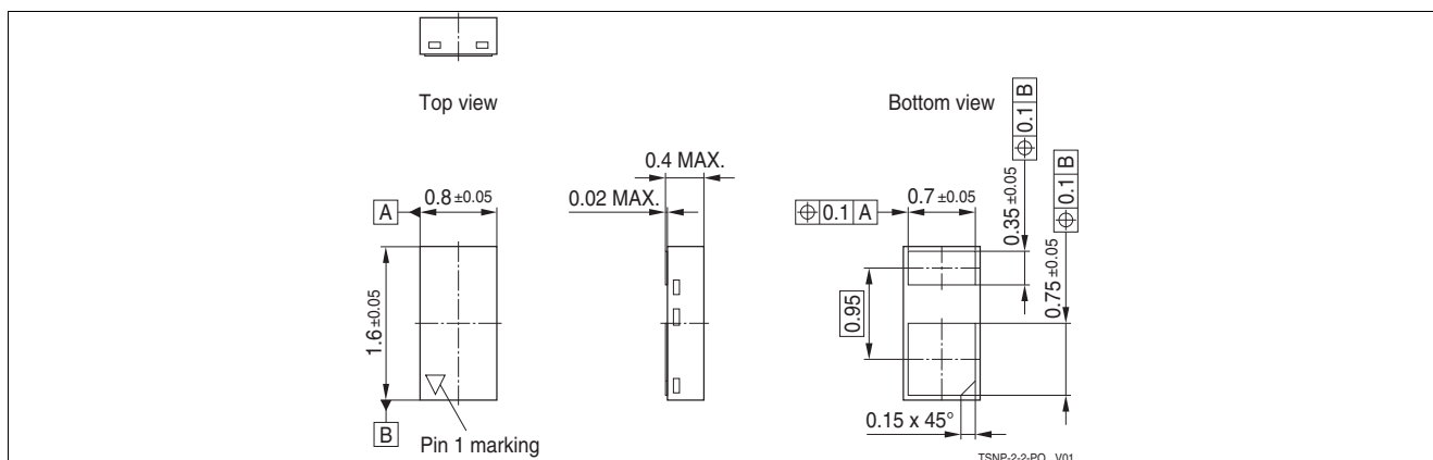
Figure 5-1 TSNP-2-2: Package outline
