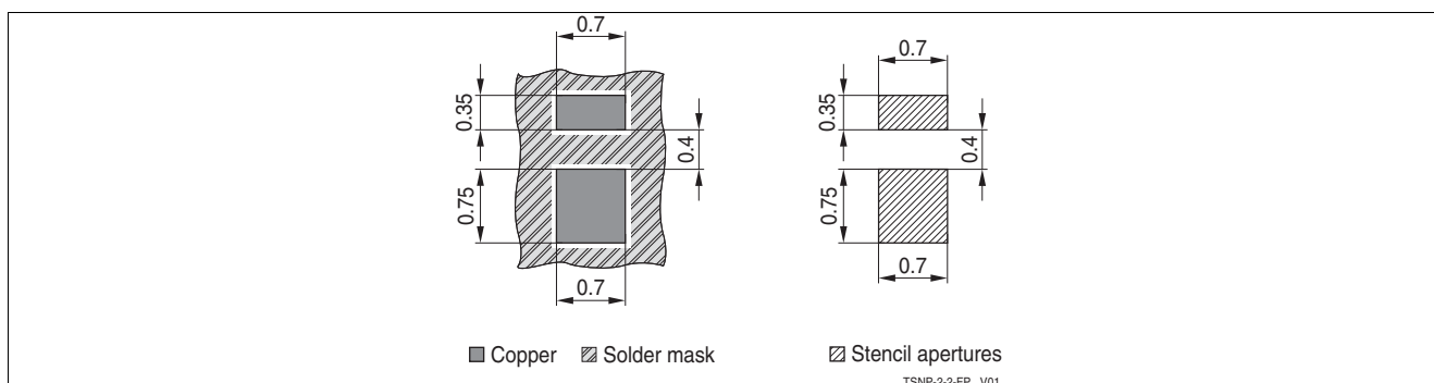
Figure 5-2 TSNP-2-2: Footprint
