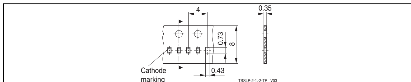
Figure 13 PG-TSSLP-2-1: Packing
