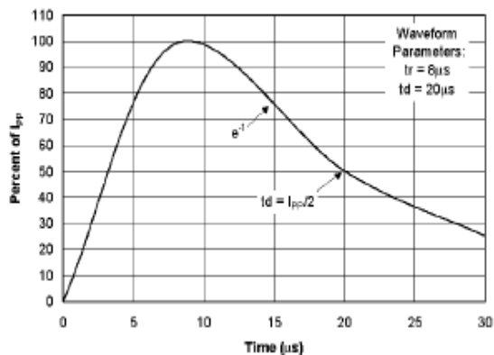
Pulse Waveform
