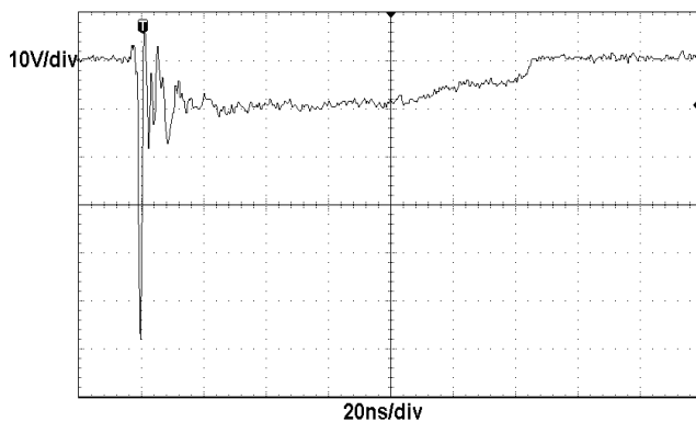
ESD clamping
