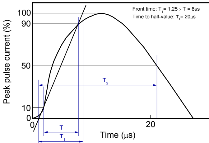
8/20 \mu\text{s} waveform per IEC61000-4-5
