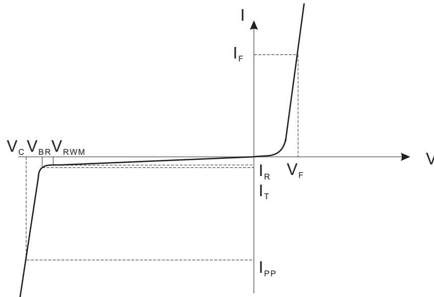
Uni-Directional TVS
